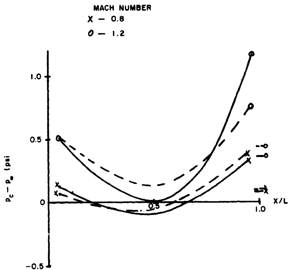
Figure 12. Comparison of Static Pressure Distribution for the Single Cavity with Doors (----) and without Doors (—) for 30,000-Foot Altitude
