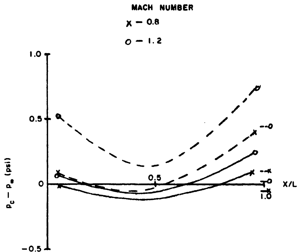
Figure 14. Comparison of the Static Pressure Distribution for the Single Cavity with Doors Configuration with (—) and without (-----) a Ramp and Spoiler for 30,000-Foot Altitude
