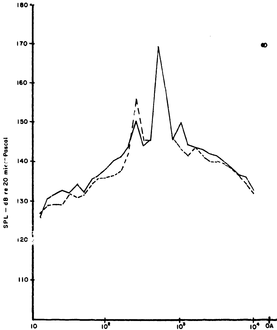
Figure 29. Comparison of the Spectra from the Single Cavity with (-----) and without (——) Doors for Mach Number 1.2 and 30,000-Foot Altitude
