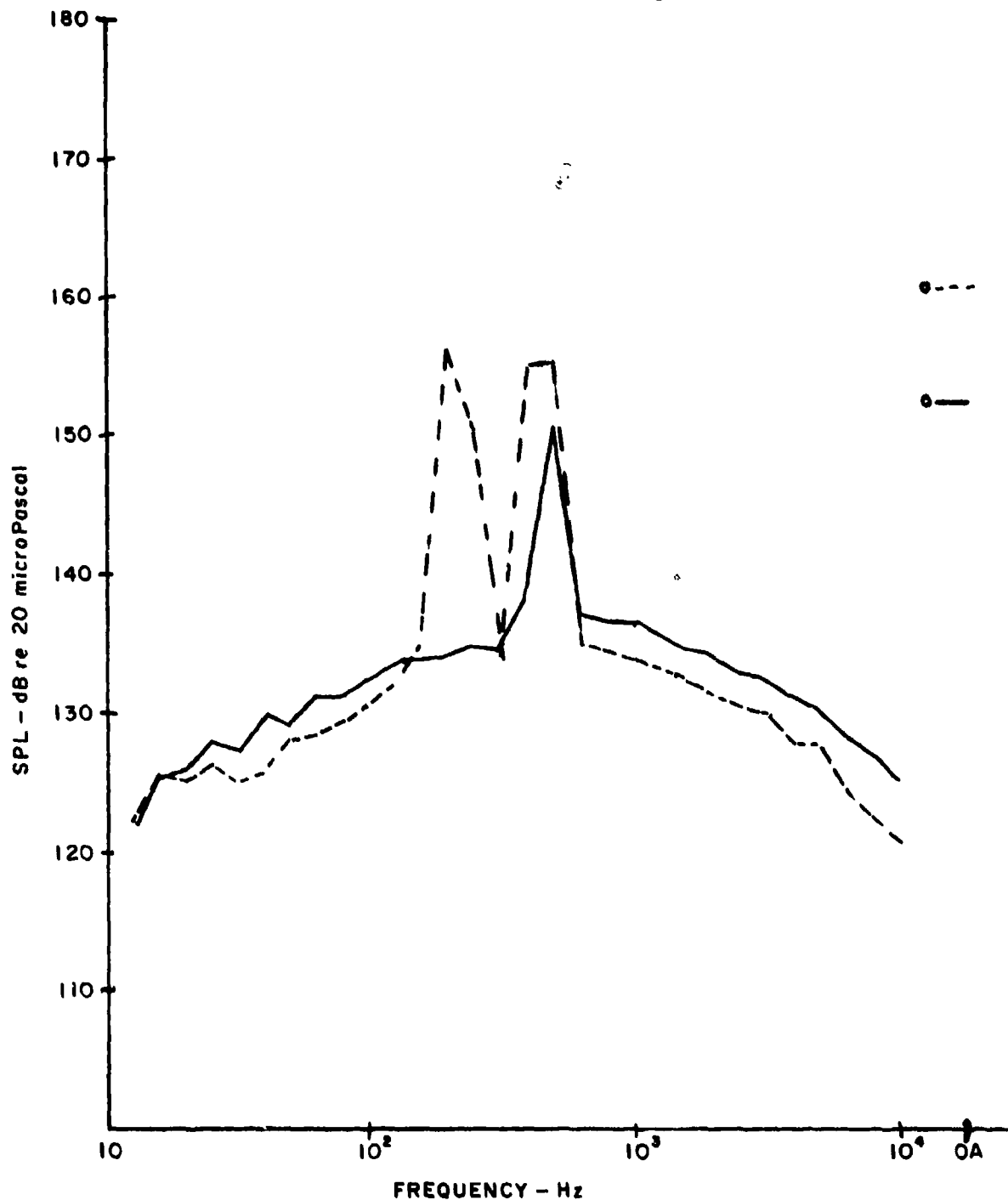
Figure 34. Comparison of the Spectra from the Single Cavity with Doors Configuration with (—) and without (-----) a Ramp and Airfoil for Mach Number 0.8 and 30,000-Foot Altitude
