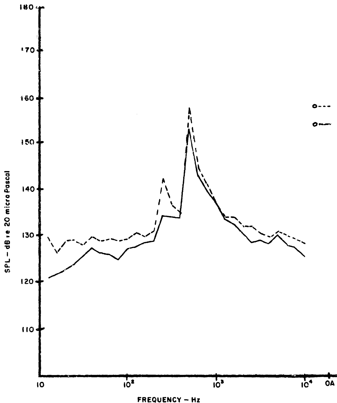
Figure 38. Comparison of the Spectra from the Single Cavity with Doors and Ramp (—) and the Front Cavity with Doors and Ramp (-----) for Mach Number 1.2 and 30,000-Foot Altitude
