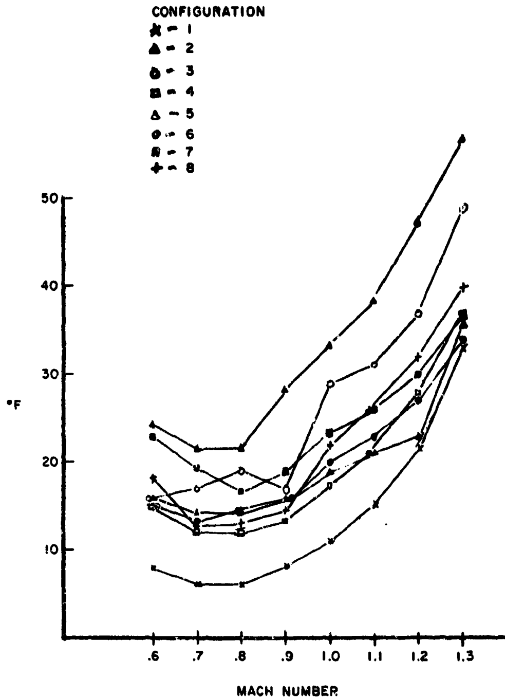
Figure 8. Comparison of the Temperature for Each of the Configurations for the 30,000-Foot Altitude
