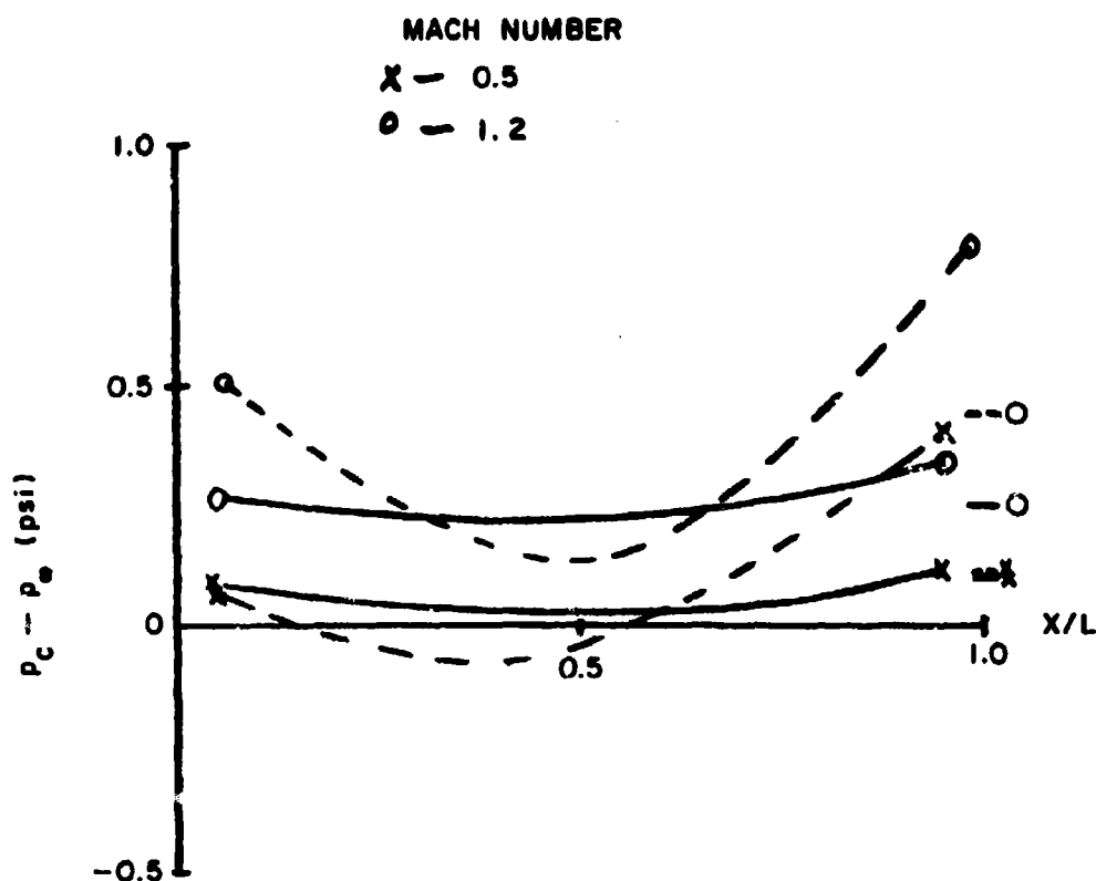
Figure 13. Comparison of the Static Pressure Distribution for the Single Cavity with Doors Configuration with a Ramp (—) and without a Ramp (----) for 30,000-Foot Altitude
