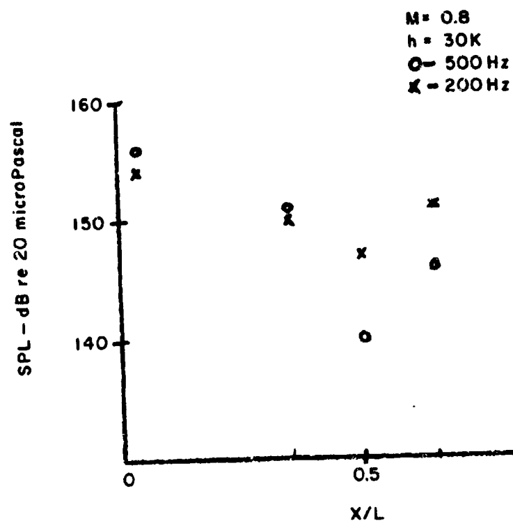
Figure 24. Longitudinal variation of the Modal Frequency Amplitudes
