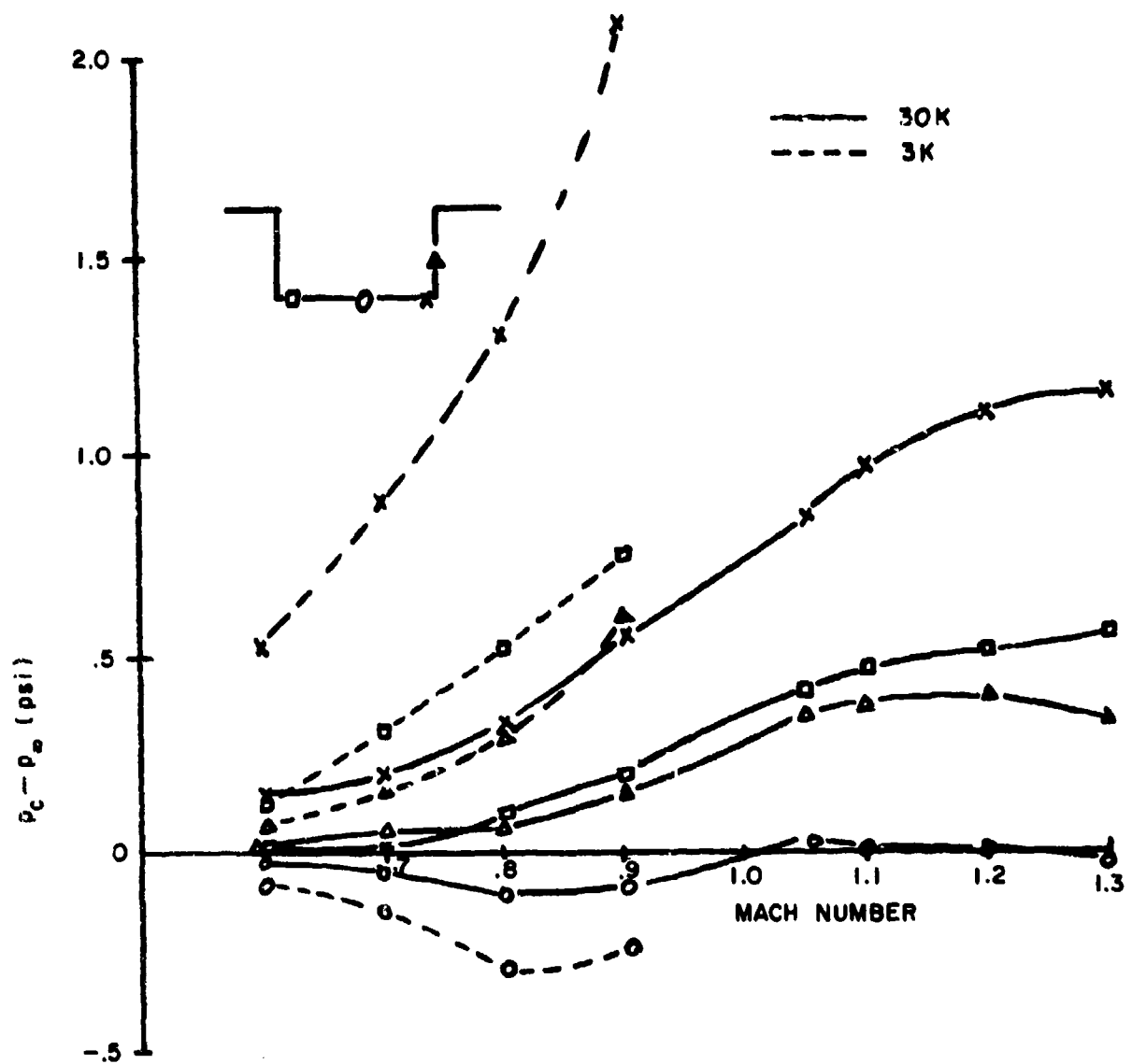
Figure 9. Static Pressure for the Clean Single-Cavity Configuration
