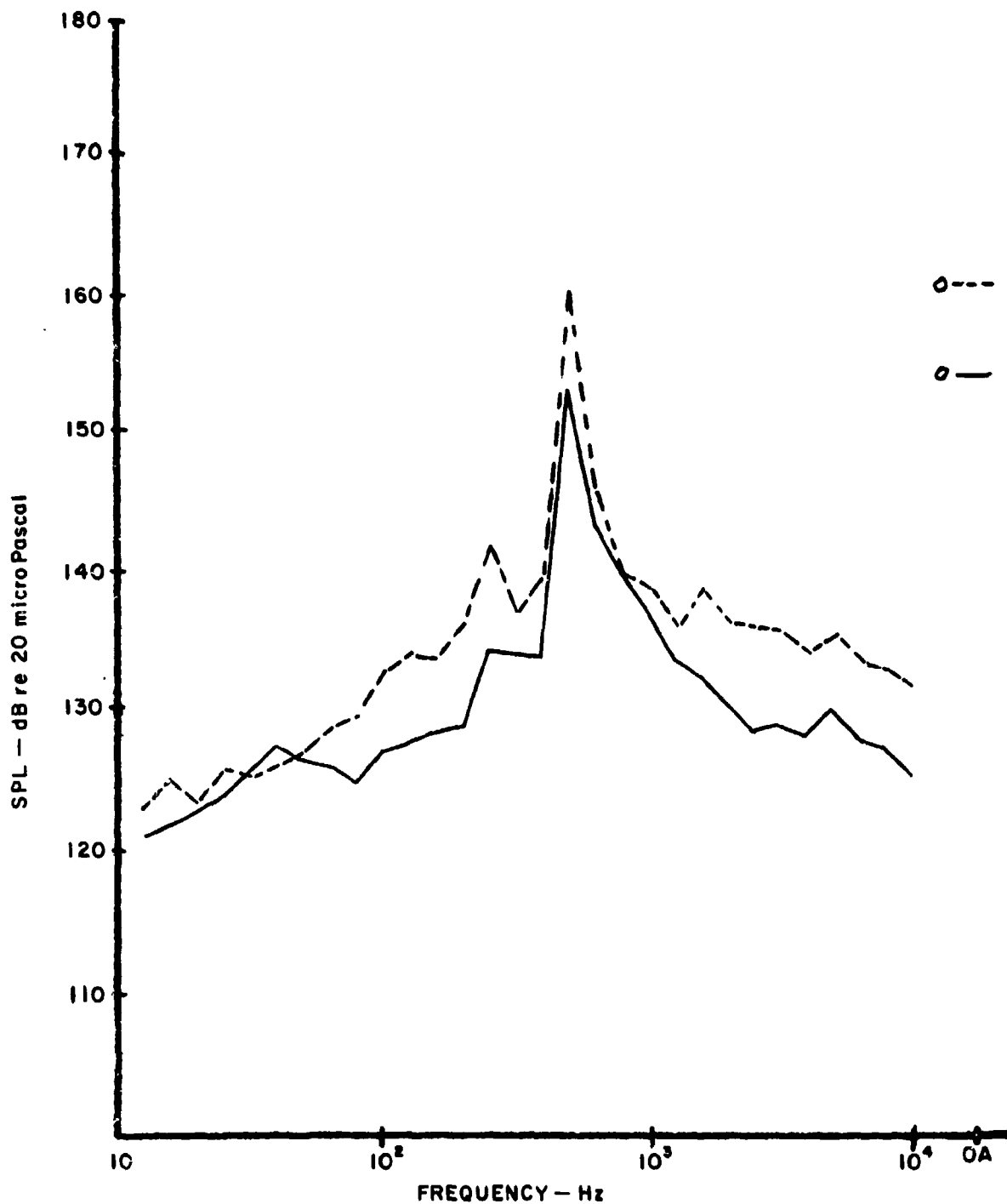
Figure 39. Comparison of the Spectra from the Single Cavity with Doors and Ramp (—) and the Rear Cavity with Doors and Ramp (----) for Mach Number 1.2 and 30,000-Foot Altitude
