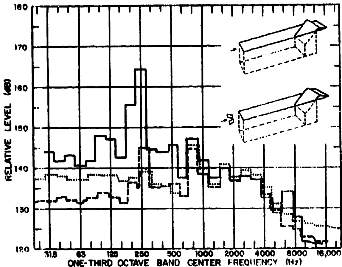
Figure 21. Effect of Training-Edge Slant with and without Upstream Spoilers on Leading-Edge Bulkhead Pressure Signal: M_\infty = 0.8 ; L/D = 2.3 (continuous line refers to unmodified cavity; dashed line refers to trailing edge slant only; dotted line refers to combination of trailing-edge slant and upstream spoilers)
