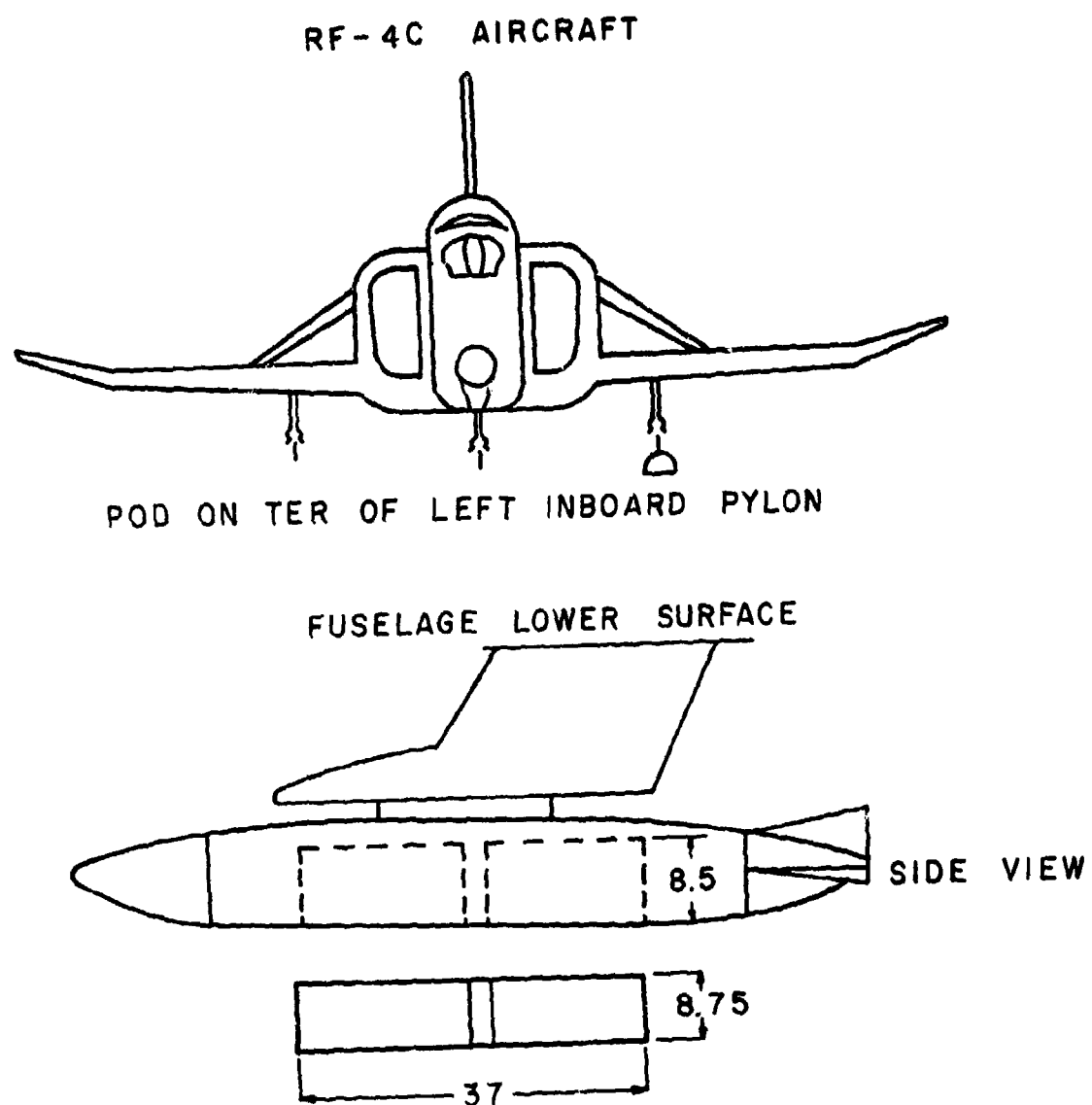
Figure 7. Modified SUU-41 Pod
