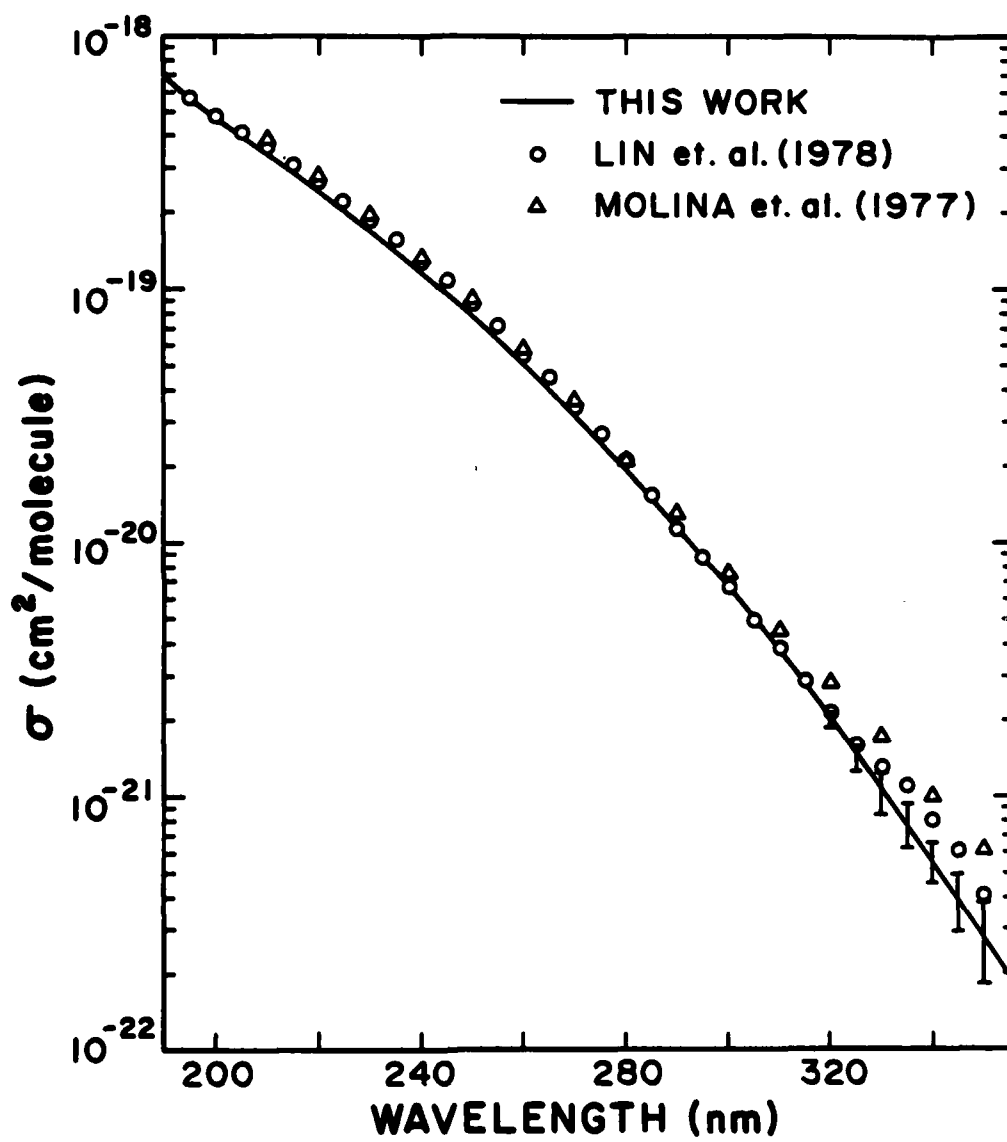
FIGURE 2. UV Spectrum of \text{H}_2\text{O}_2 Vapor.
