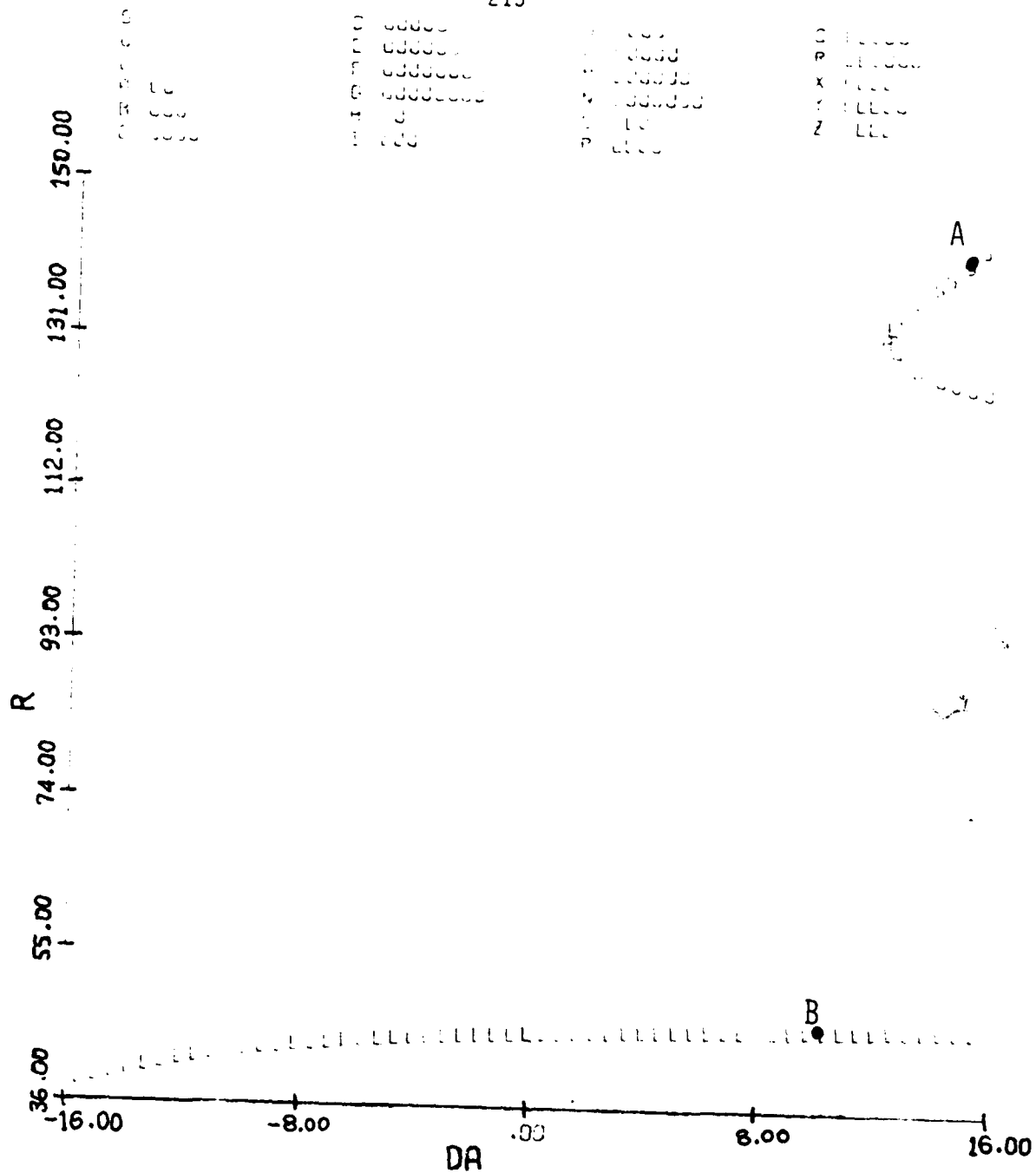
FIGURE 3.50(a) Equilibrium Surface: r, \alpha, p vs. \delta a \delta e = 0^\circ , \delta r = -25^\circ , V = 600 fps, g = 0
