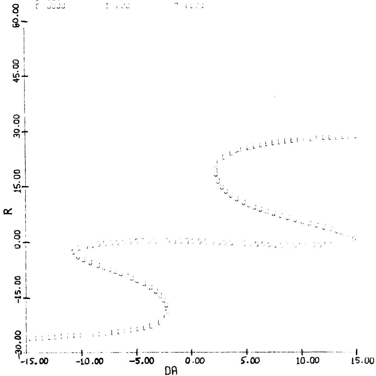
FIGURE 3.12(a) Equilibrium Surface: r, \alpha, p vs. \delta a \delta e = -11^\circ , \delta r = 0^\circ , V = 600 fps, g = 0
