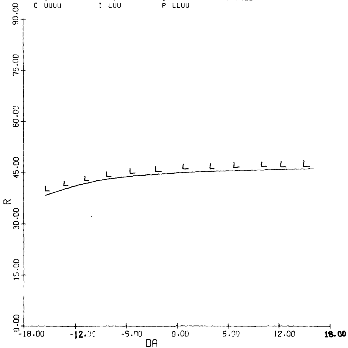
Figure 3.22(a) Equilibrium Surface: r, \alpha, p vs. \delta a V = 600 fps, g = 0
