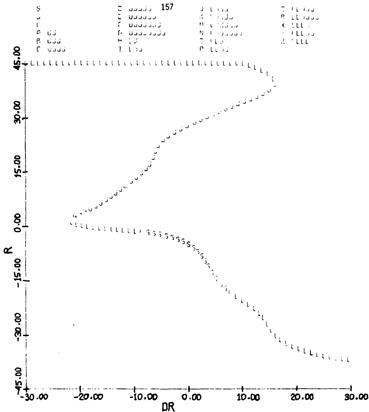
FIGURE 3.25(a) Equilibrium Surface: r, \alpha, p vs. \delta r \delta a = 15^\circ , \delta e = 0^\circ , V = 600 fps, g = 0
