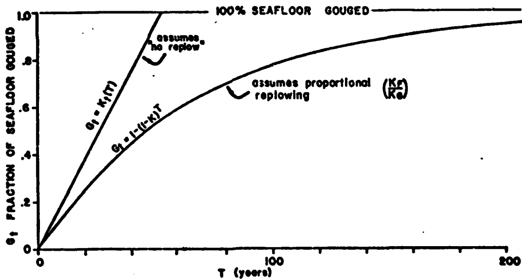
b. Graph illustrating fraction of the sea floor disrupted by ice ( G_t ) as a function of time, assuming no reflow K_t(T) and proportional reflowing 1 - (1 - K)^T .
