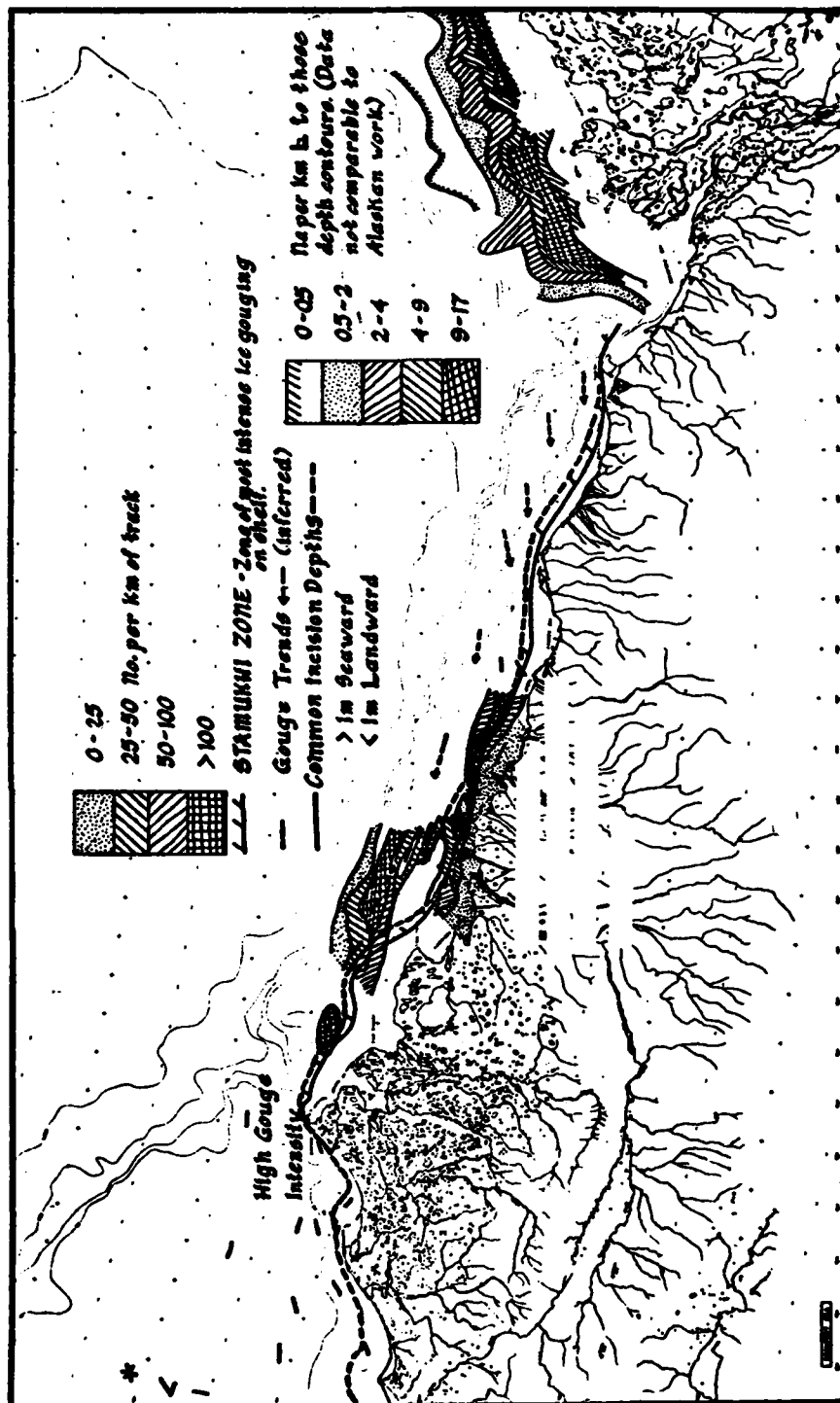
Figure 17. Ice gouging of sediments. (From OCSEAP 1978.)
