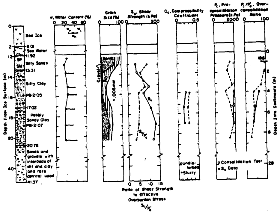
Figure 5. Drill hole log and engineering properties for site PB-2. (From Sellmann and Chamberlain 1979.)
