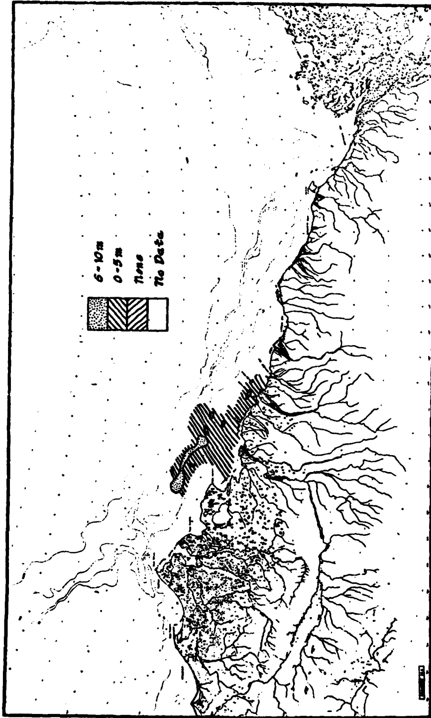
Figure 2. Thickness of recent (Holocene) sediments mapped to date. (From OCSEAP 1978.)
