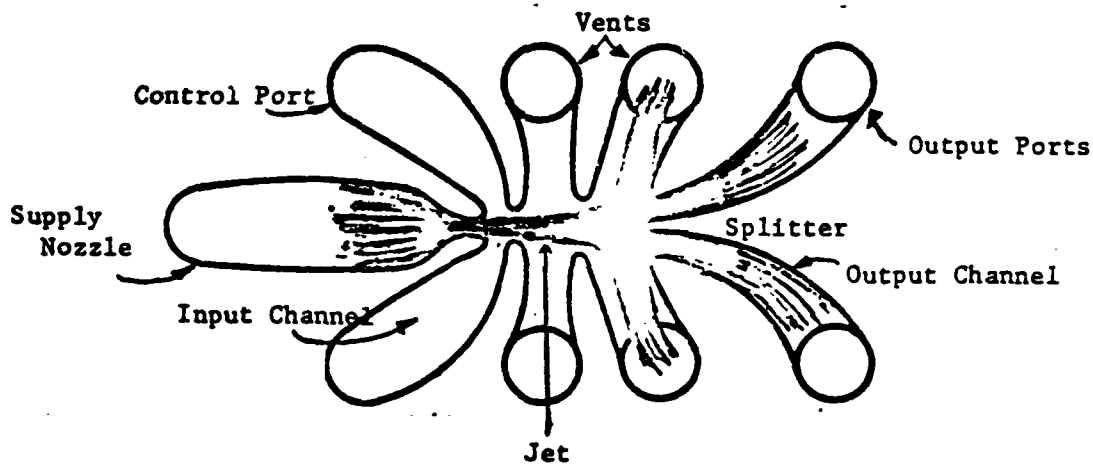
Figure 10. Schematic of a laminar proportional amplifier.
