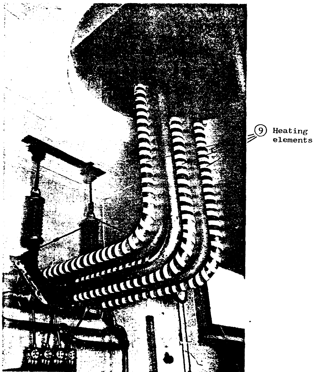
Figure 10. Heated tube array, lower part, with heating elements applied but without insulation. Numbers in circles refer to item list in Figure 5.
