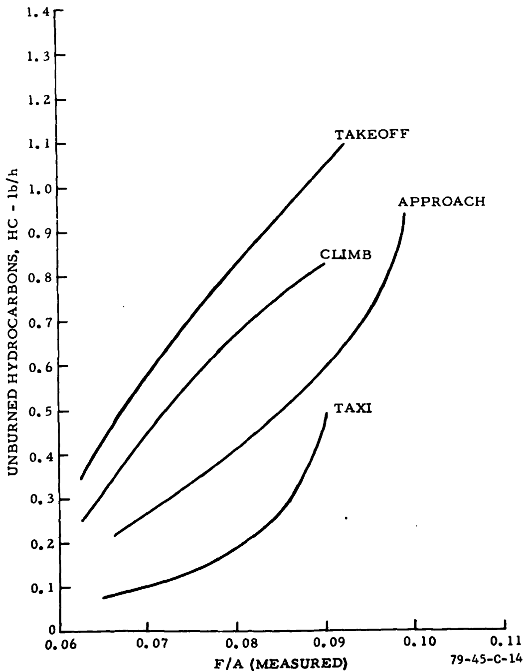
FIGURE C-14. NOMINAL SEA LEVEL STANDARD DAY EMISSIONS CHARACTERISTICS FOR AN AVCO LYCOMING O-320-DIAD ENGINE--UNBURNED HYDROCARBONS
