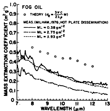
Figure 11. Same as figure 10 except for the 7μm to 13μm spectral region. The overprediction of extinction according to the linear relation (5) (open circles) is partially caused by inaccuracy of the Q_e = cx approximation (e.g., figure A-7). The good agreement of the measurements for the widely differing optical depths (solid and dashed curves) suggests multiple scatter contributions are not significant. Alternatively, experimental errors in the extinction-to-mass ratio may be so large as to obfuscate multiple scatter contributions.
