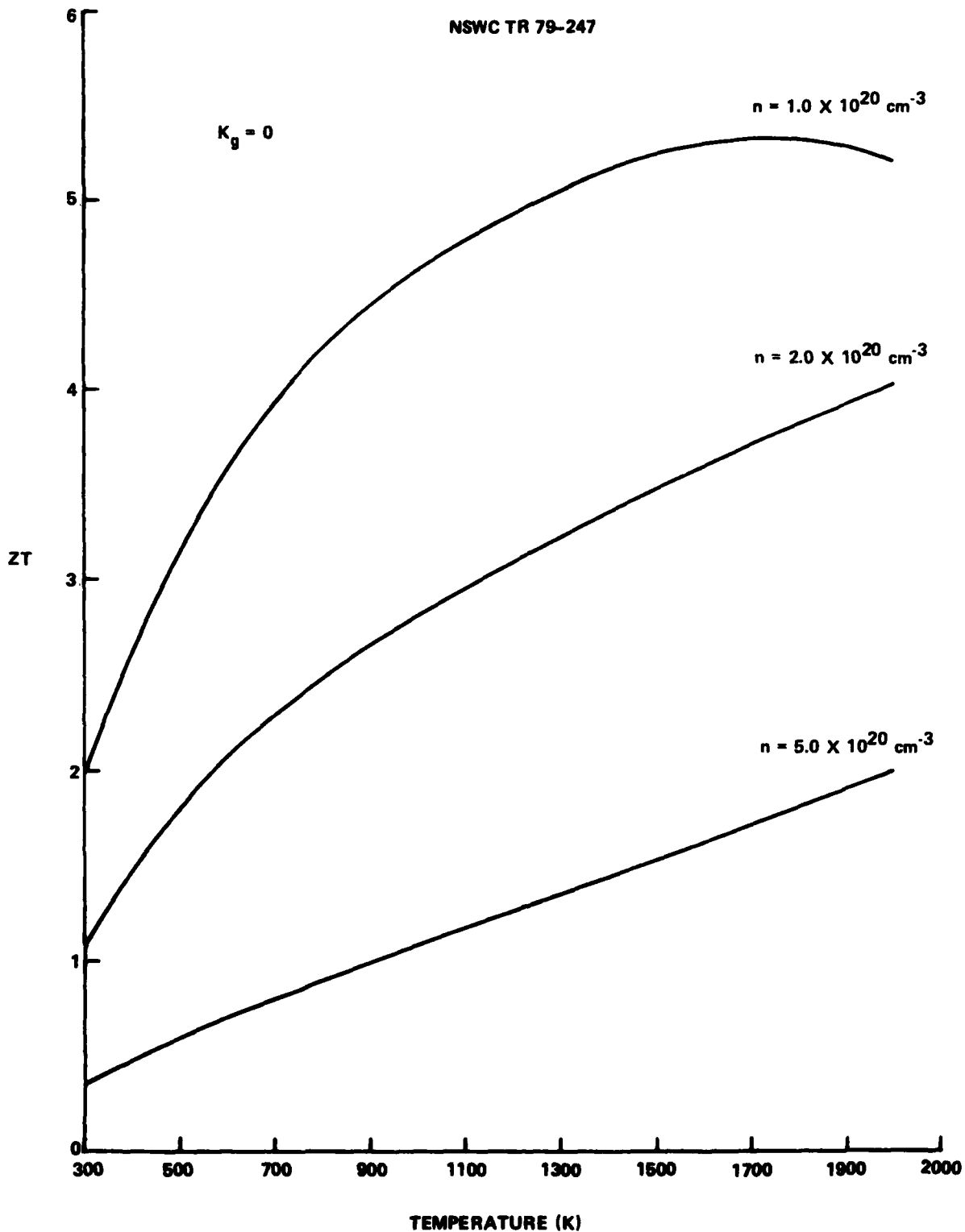
FIGURE 3 THE THERMOELECTRIC EFFICIENCY ZT vs. TEMPERATURE T AND CARRIER DENSITY n FOR LATTICE THERMAL CONDUCTIVITY K_g = 0 . THE THEORETICAL PHOTON THERMAL CONDUCTIVITY K_r HAS BEEN INCLUDED IN THE CALCULATIONS
