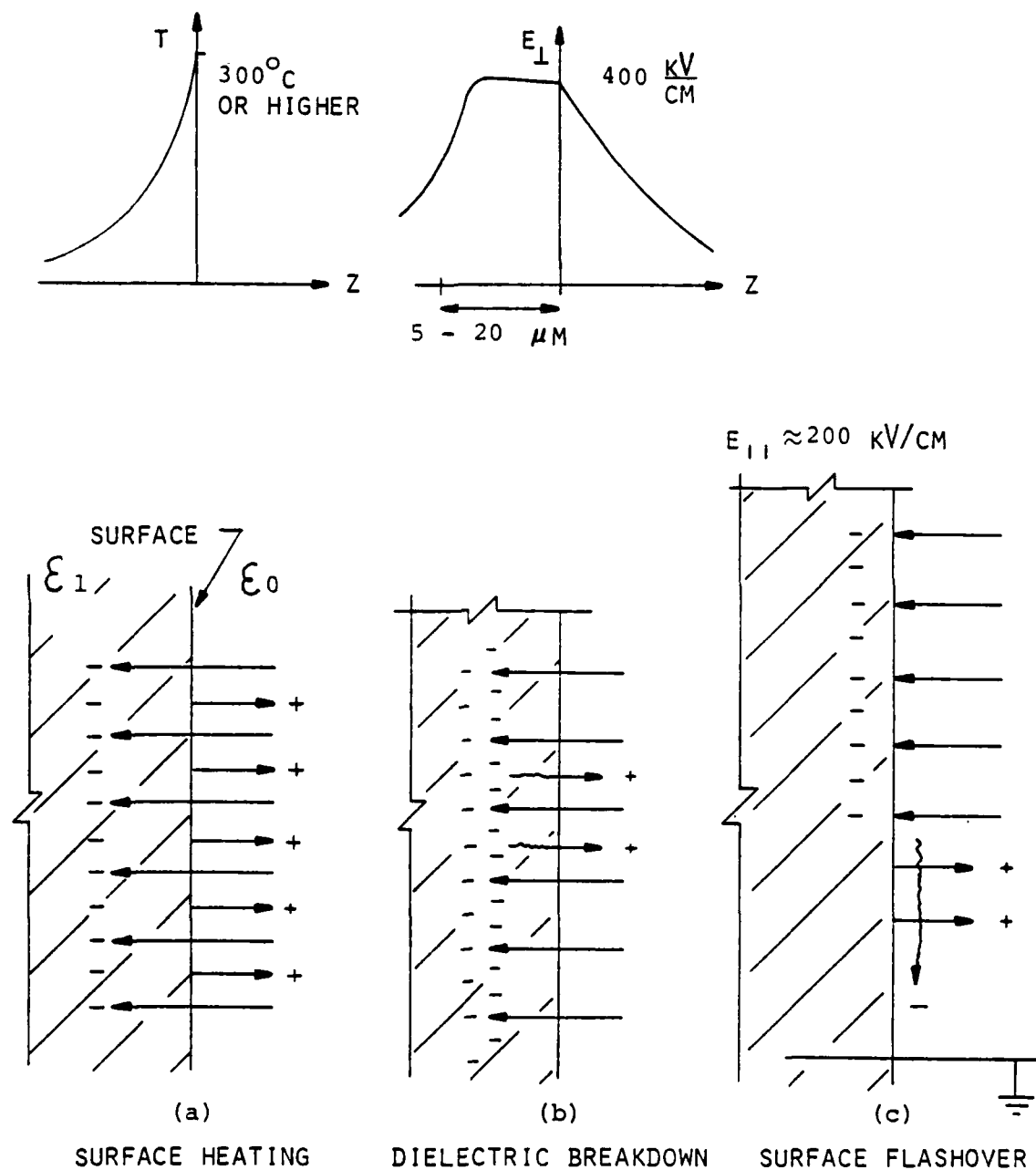
Figure 11. How Ions Can be Released from Surface of Dielectric Material.
