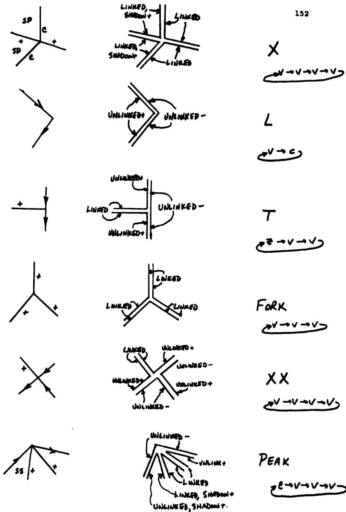
Figure D.1. Some Examples of Waltz Labelings and H-C Labelings
