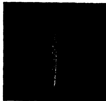
Psuedo- Hueckel
