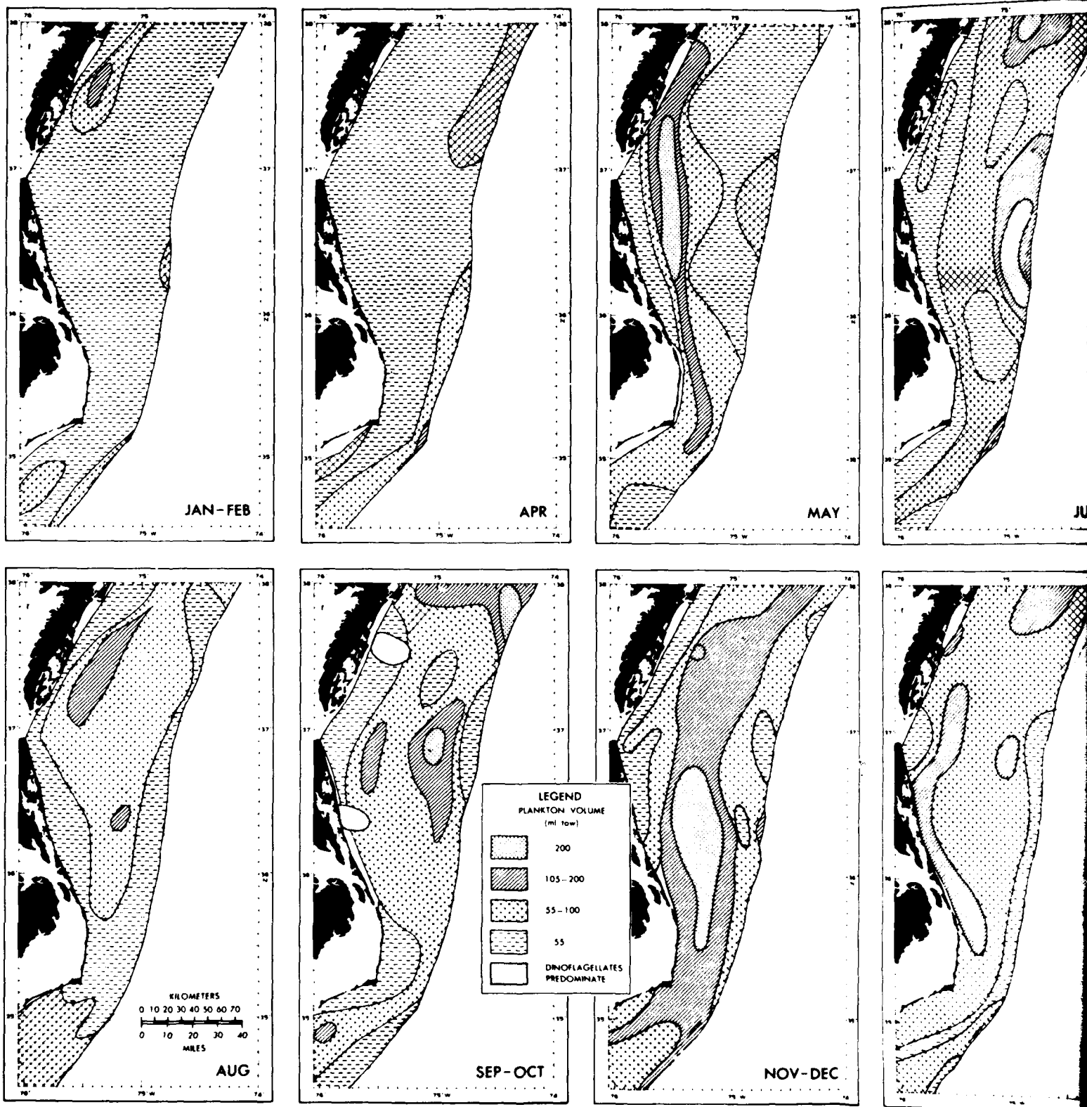
FIGURE 30. PLANKTON VOLUME FOR SHALLOW WATER—CONTINENTAL SHELF (1 TO 100 FM)
