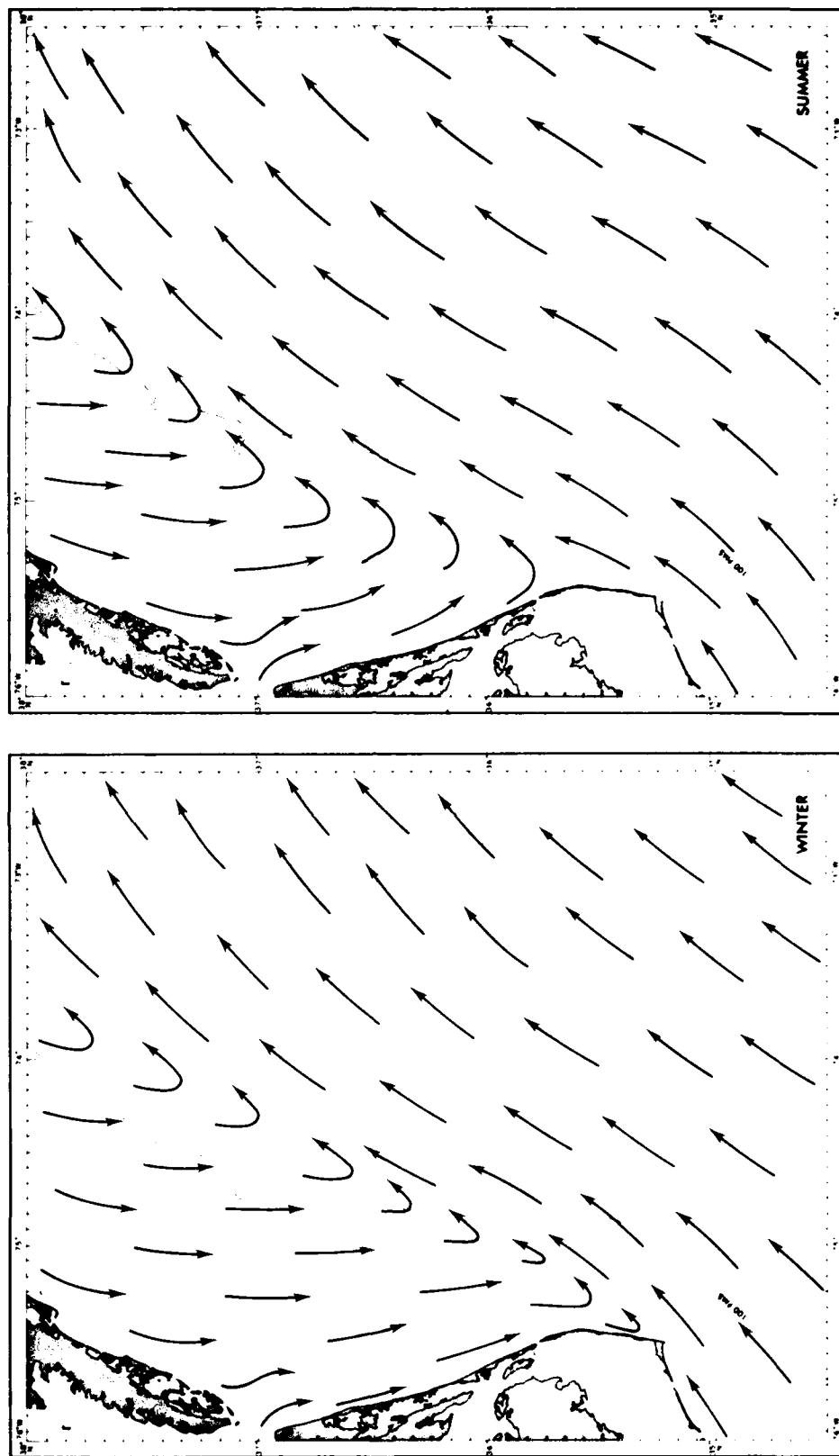
FIGURE 3. SURFACE CURRENTS
