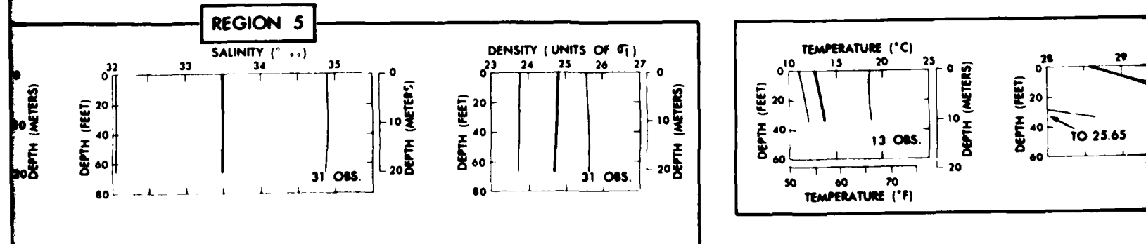
FIGURE 17. TYPICAL TRACES AND RANGES OF TEMPERATURE, SALINITY, AND DENSITY,
