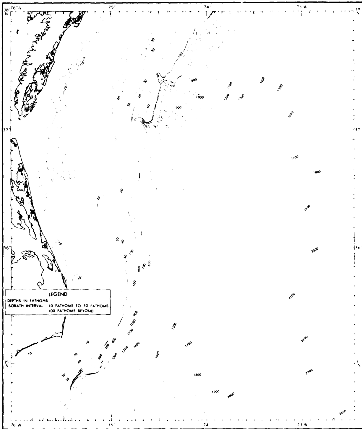
FIGURE 20. BATHYMETRY
