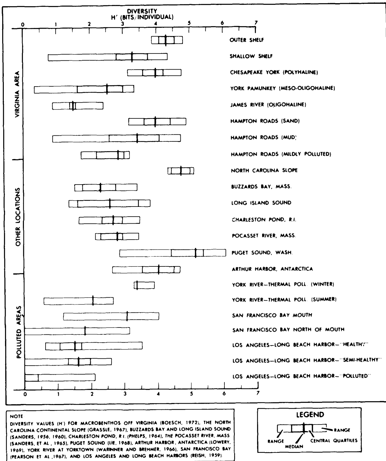
FIGURE 35. DIVERSITY VALUES FOR MACROBENTHOS OFF VIRGINIA AND OTHER AREAS
