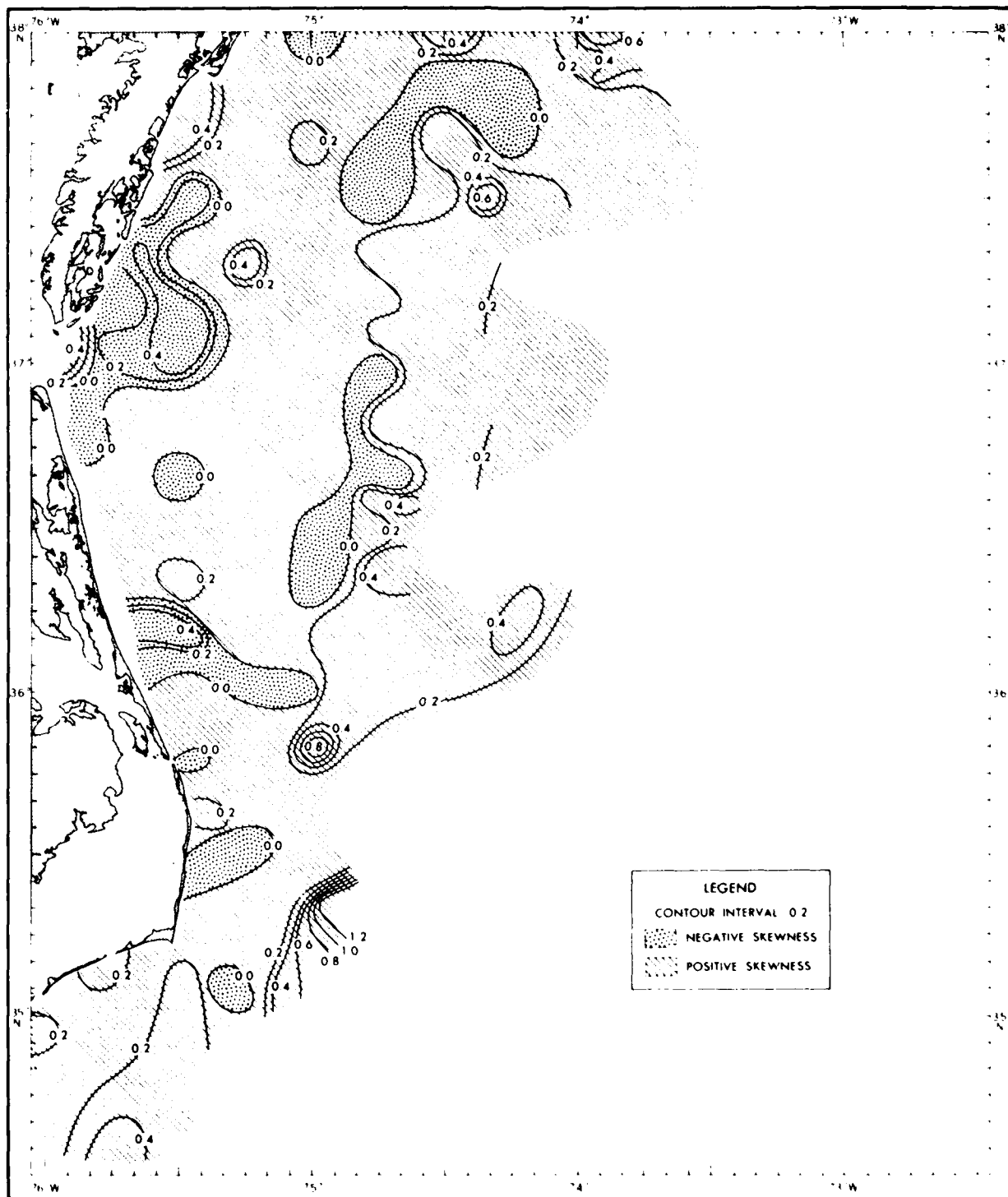
FIGURE 25 SKEWNESS
