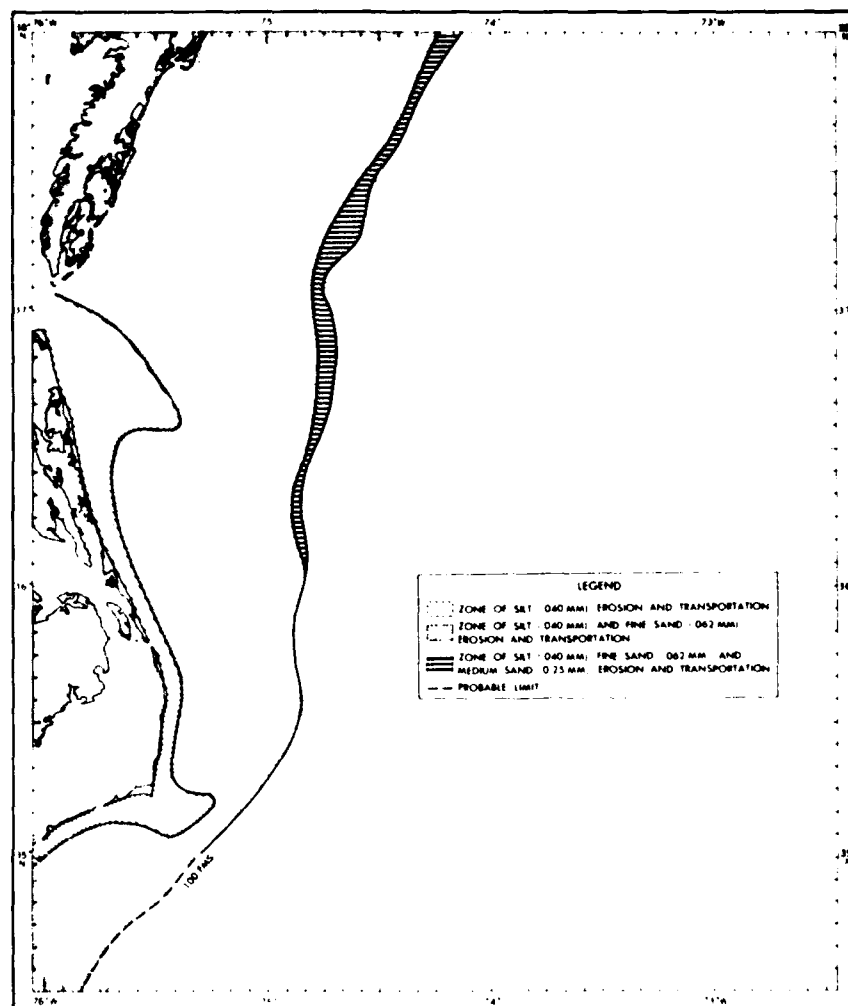
FIGURE S 7. ZONES OF SUSPENSION AND TRANSPORT RELATED TO GRAIN SIZE
