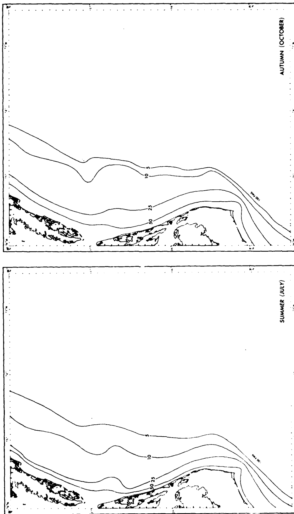
FIGURE 12 PERCENT FREQUENCY OF WAVES TOUCHING BOTTOM (CON.)
