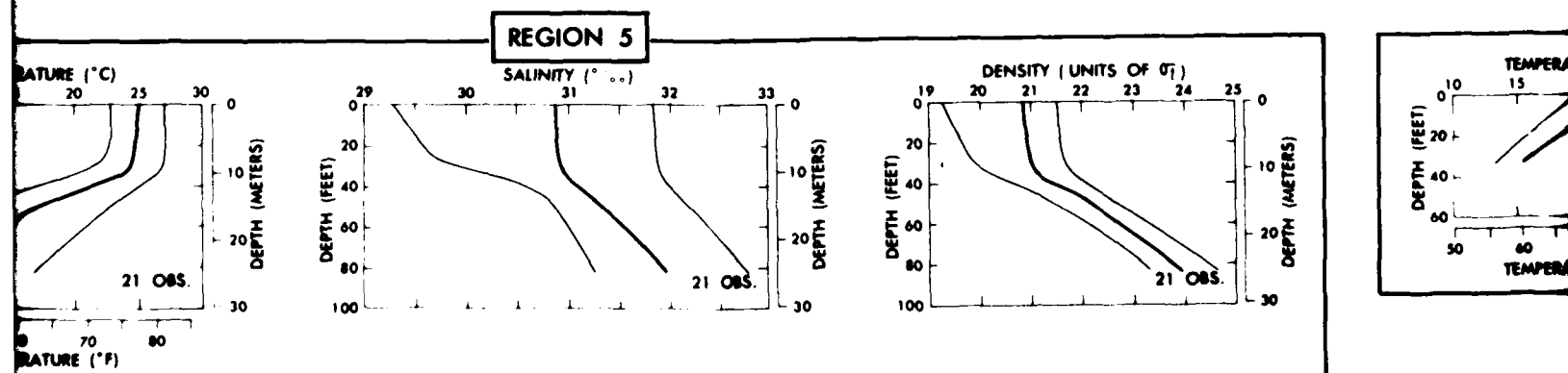
FIGURE 16. TYPICAL TRACES AND RANGES OF TEMPERATURE, SALINITY, AND DENSITY
