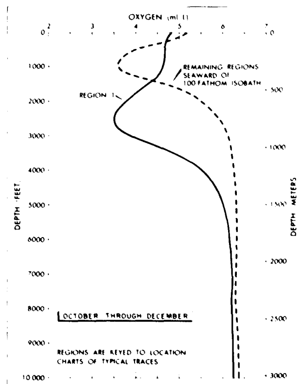
FIGURE A 7 MEAN OXYGEN TRACES
