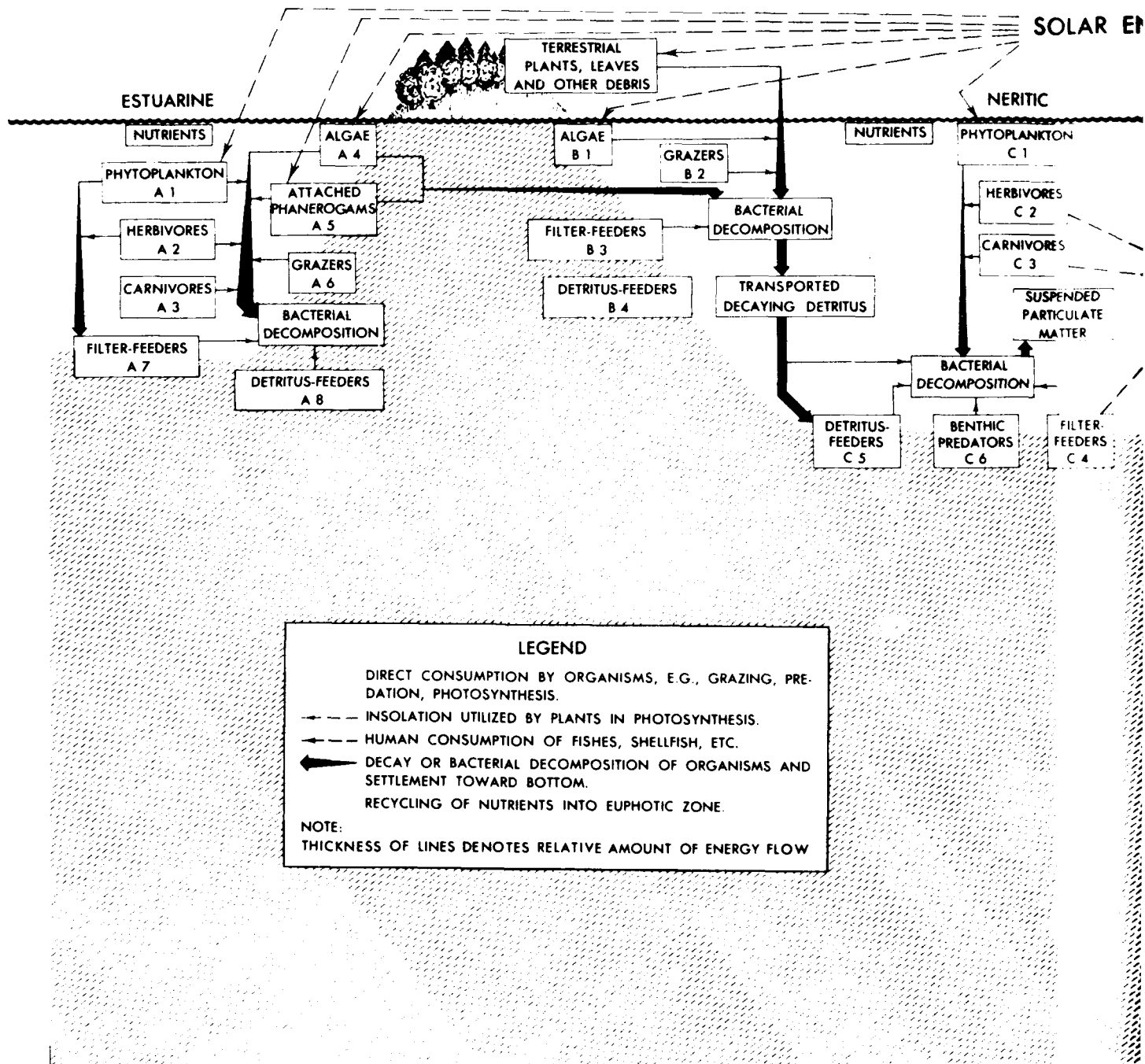
FIGURE 52. FOOD WEB AND ENERGY FLOW SUMMATION AND ORGANIC EXCHANGE BETWEEN MAJOR DEPTH ZONES (C)
