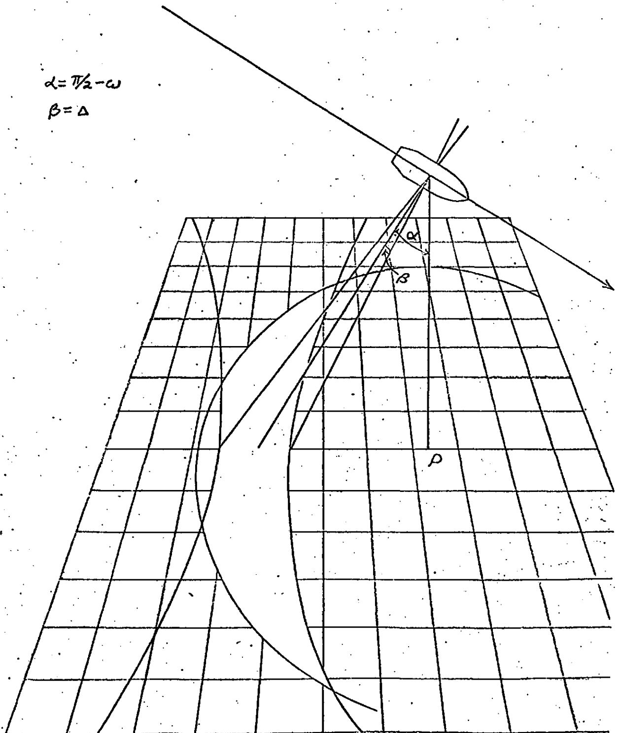
Figure 2. Geometry of a Burst over the Ground Plane (from BRL R530)
