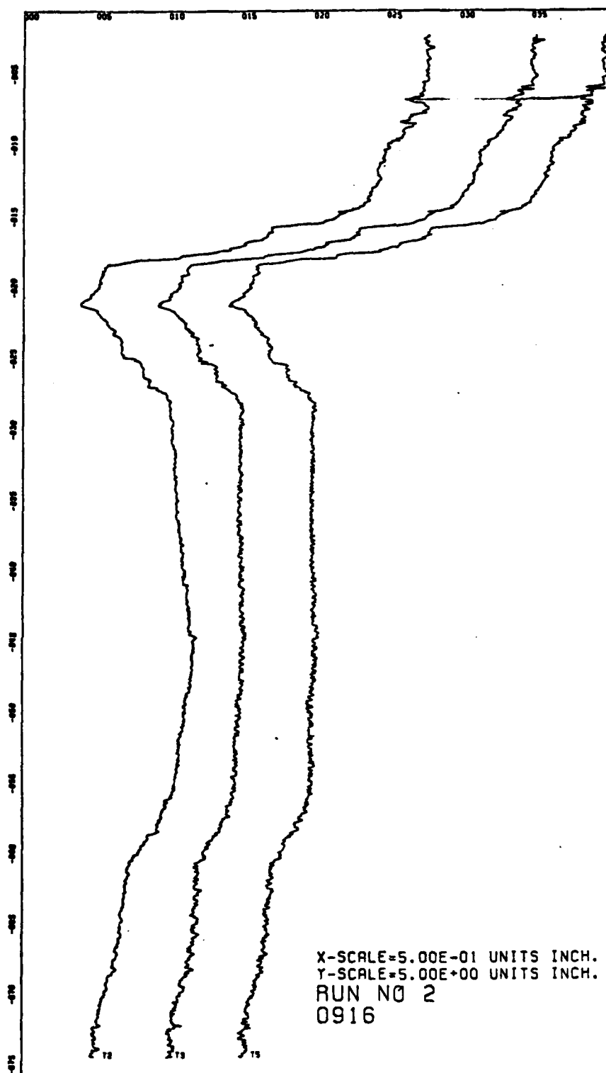
Figure 4. Microstructure Profile, 0916
