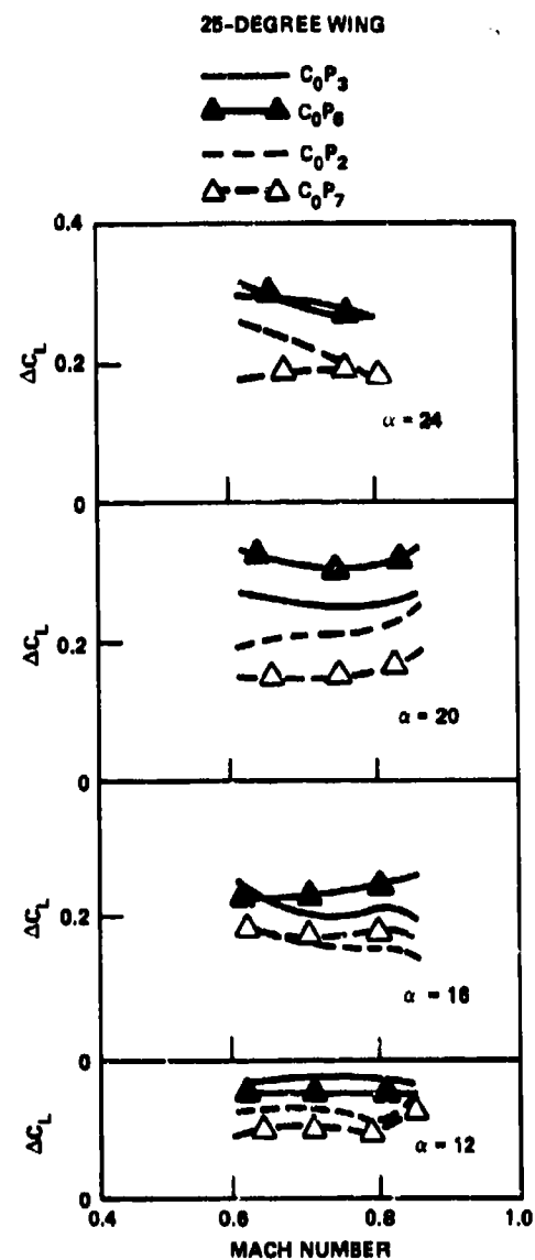
Figure 11d - Canard C_0
