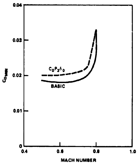
Figure 49 - Minimum Drag of the 25-Degree Wing with and without Canard
