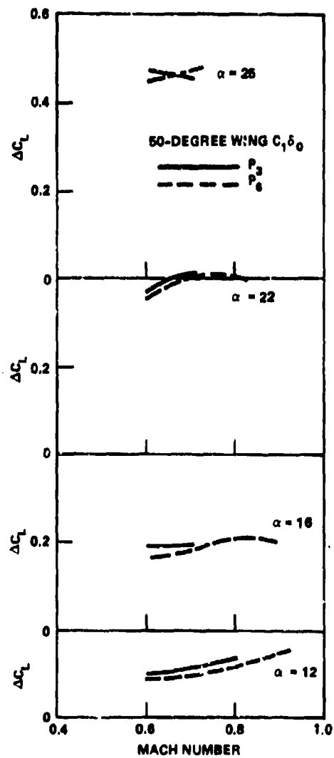
Figure 11b - Canard C_1
