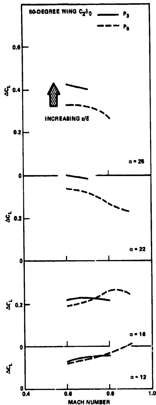
Figure 11c - Canard C_2
