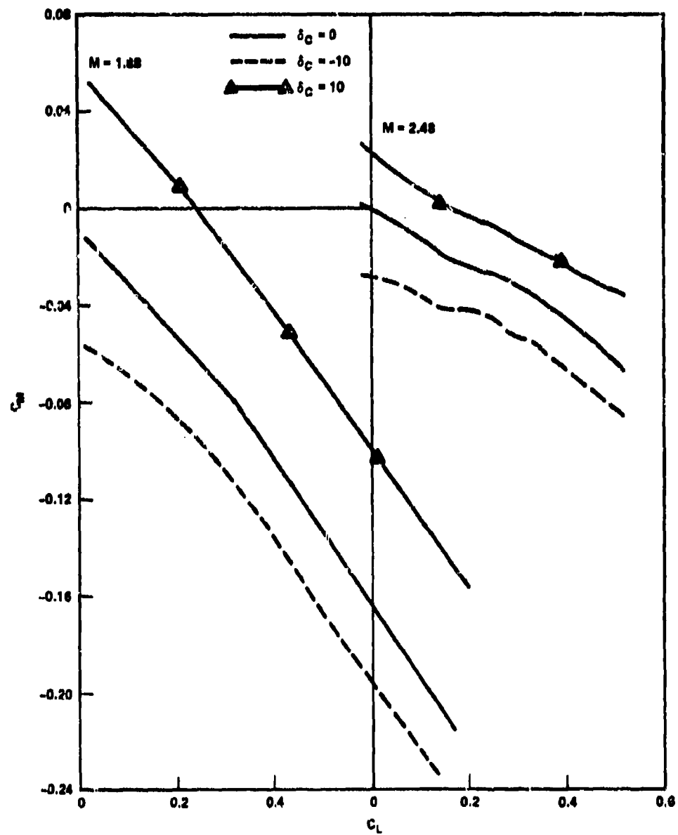
Figure 92c - Pitching Moment
