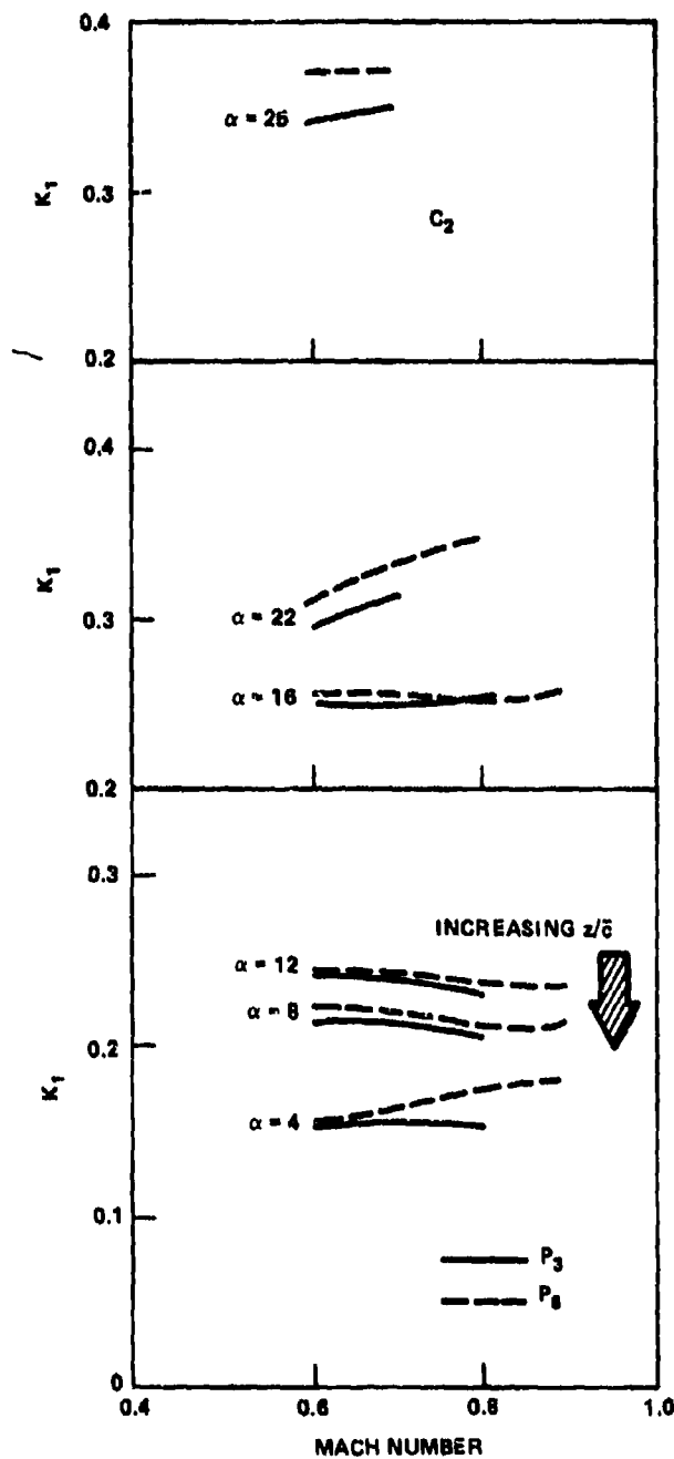
Figure 54c - Canard C_2 on 50-Degree Wing
