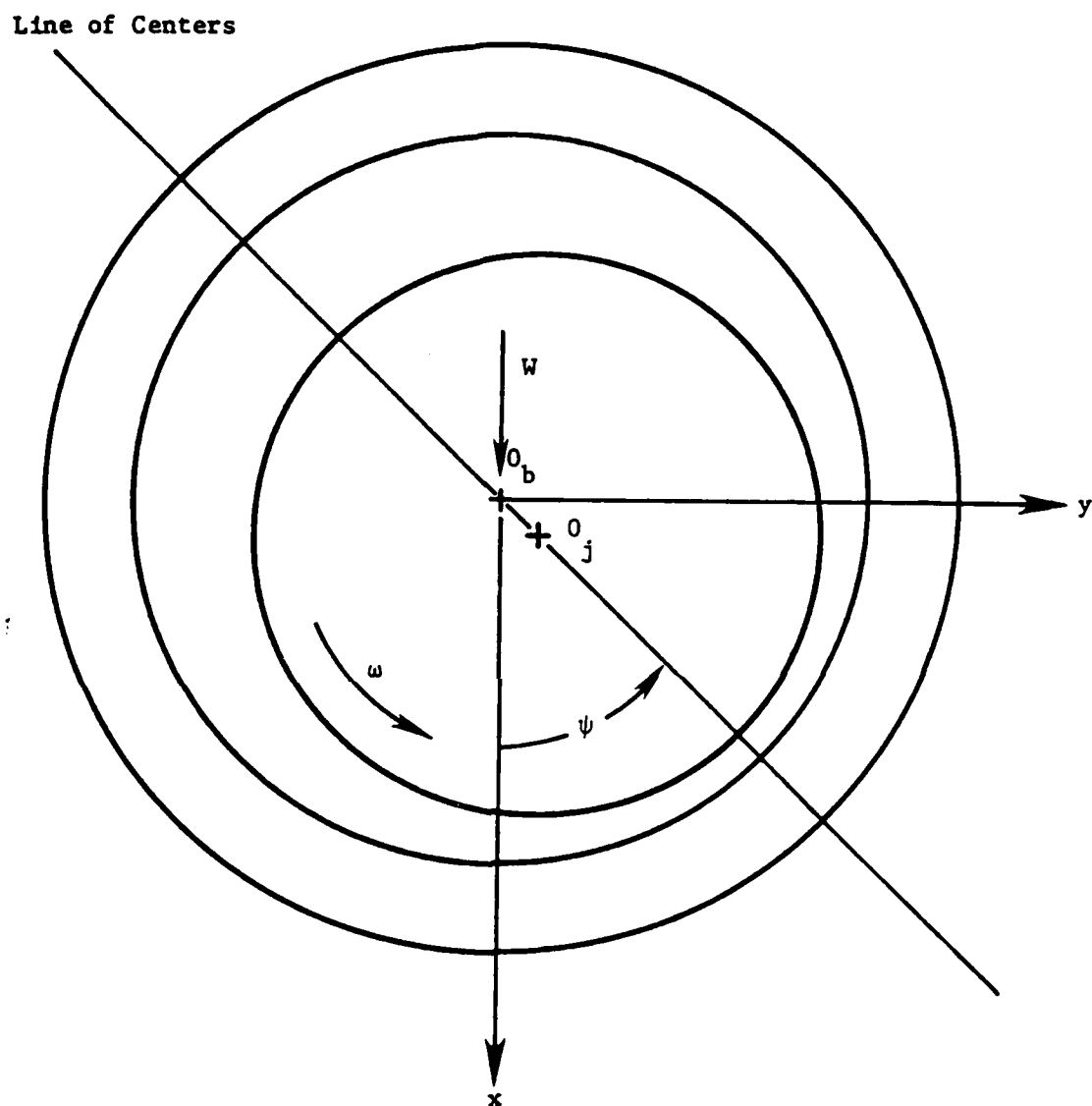
Figure 4 Plain Journal Bearing
