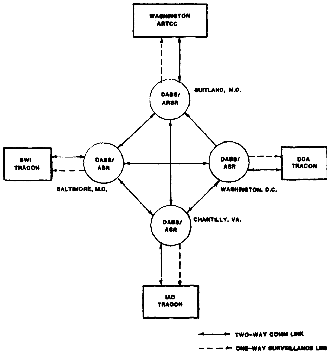
Fig. 7. DABS/ATC Configuration.
