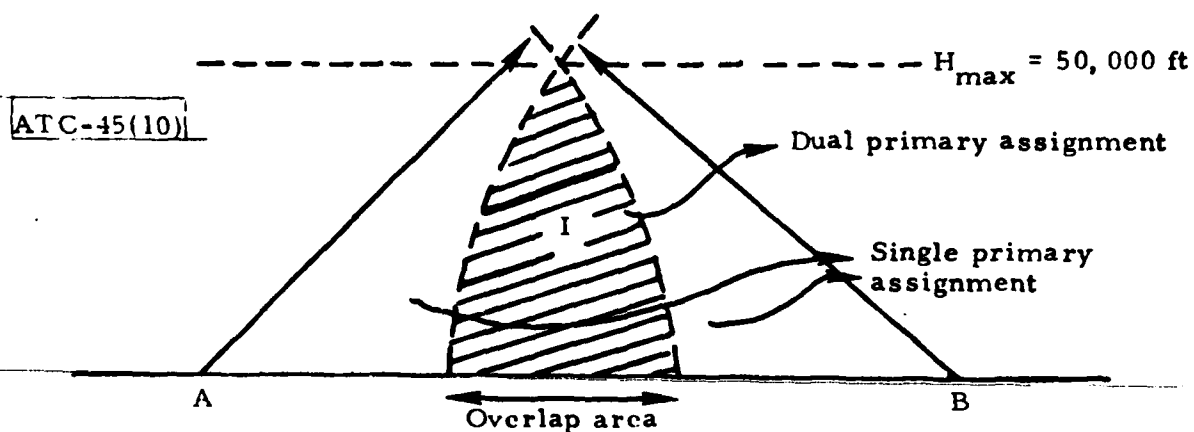
Fig. 4. Enlarged Overlap Area.
