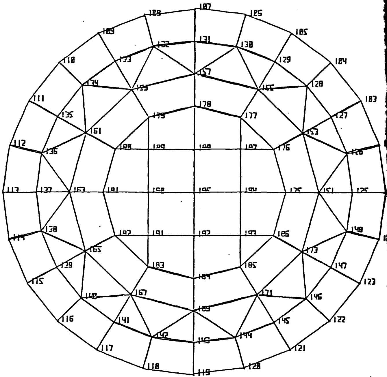
Figure 6. Level 1 with grid points labeled.
