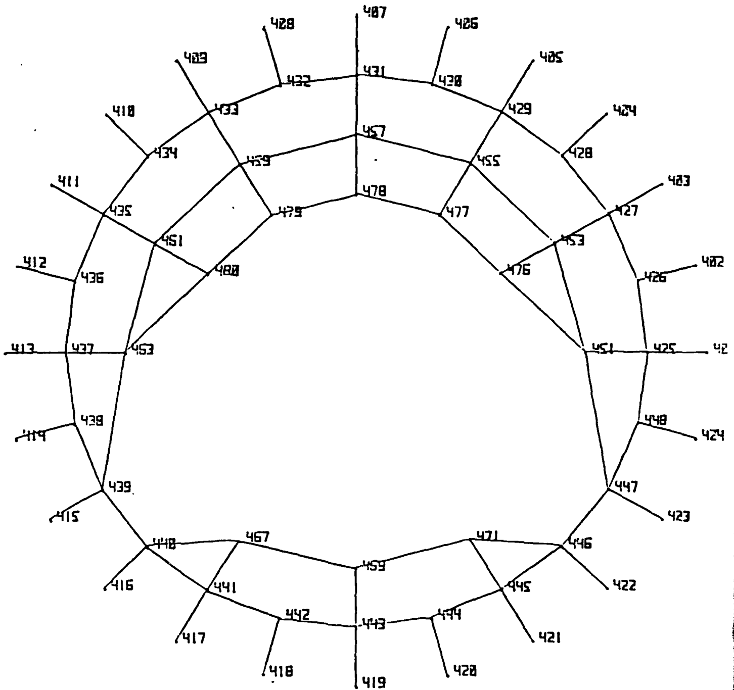
Figure 9. Level 4 with grid points labeled.
