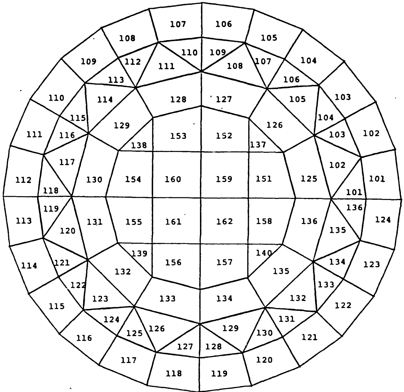
Figure 12. Level 1 quadrilateral and triangular plate element ID's. Levels 2, 3 and 6 are analogous in the 200, 300 and 400 series, respectively.
