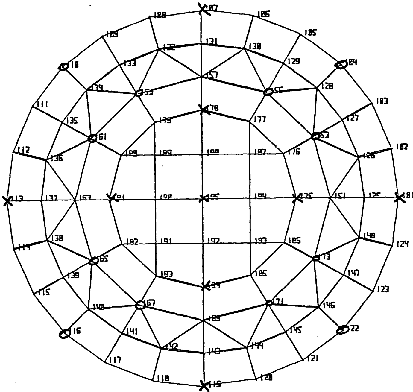
Figure 18. Plot of level 1 showing representative degrees of freedom placed in analysis set.
