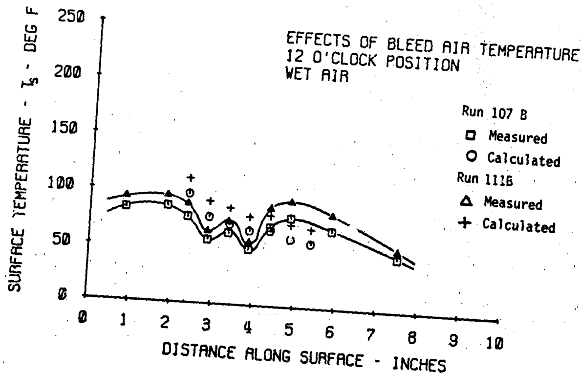
Figure 4-16 (Cont.) - Wet Air
