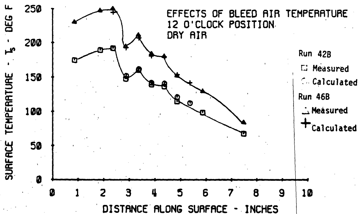
Figure 4-16 Comparison of Calculated and Measured Surface Temperature for Two Bleed Air Temperatures. - Dry Air
