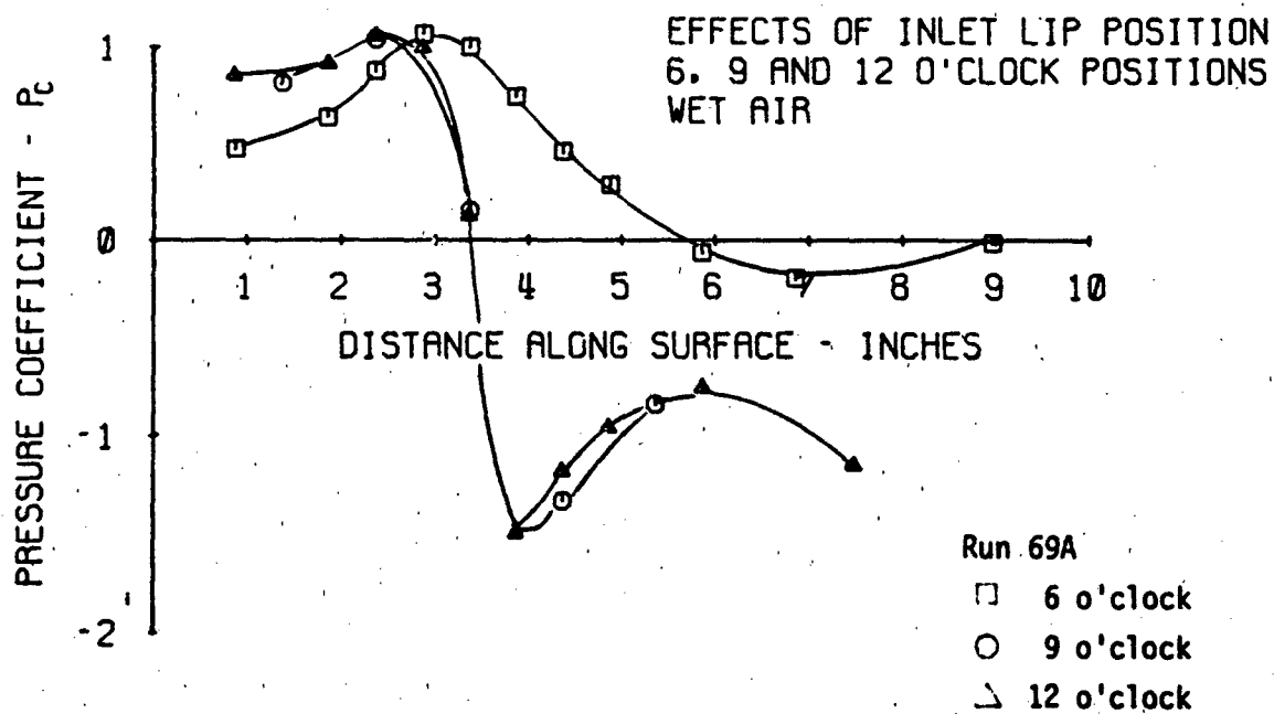
Figure 4-5 Effects of Nacelle Lip Position on Surface Pressure Coefficient
