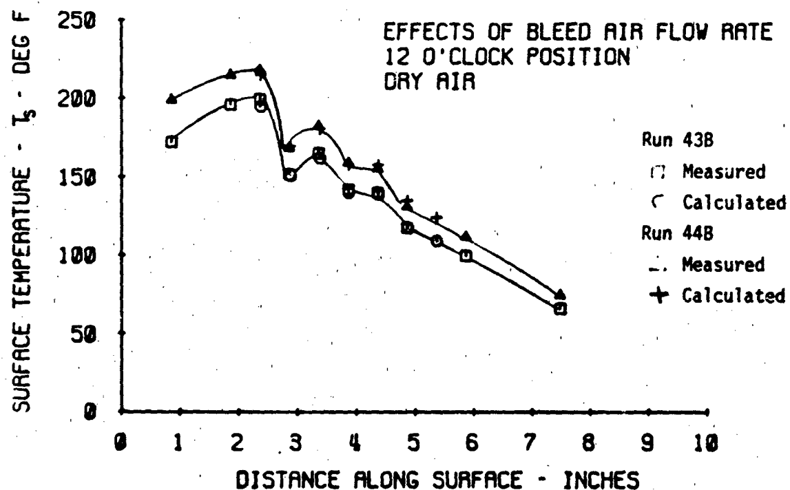
Figure 4-17 Comparison of Calculated and Measured Surface Temperature for Two Bleed Air Flow Rates.
