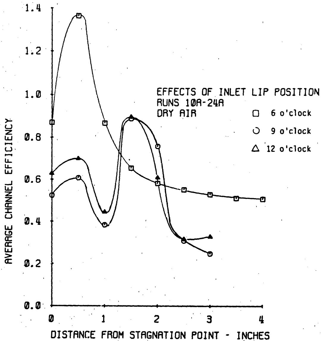
Figure 4-6 Effects of Nacelle Lip Position on Efficiency Distribution
