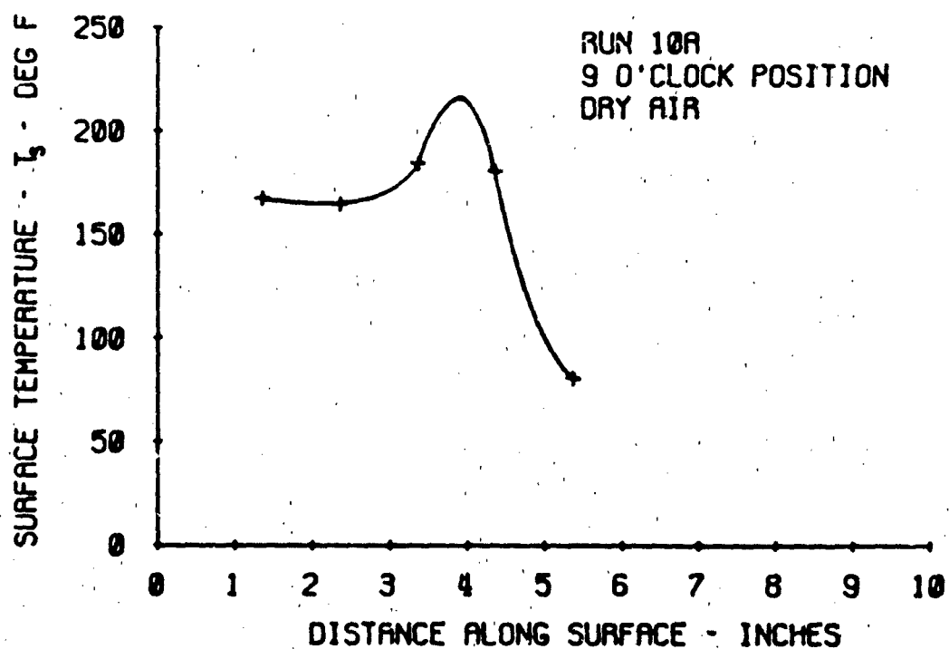
Figure 4-2 Typical Measured Surface Temperature Distribution
