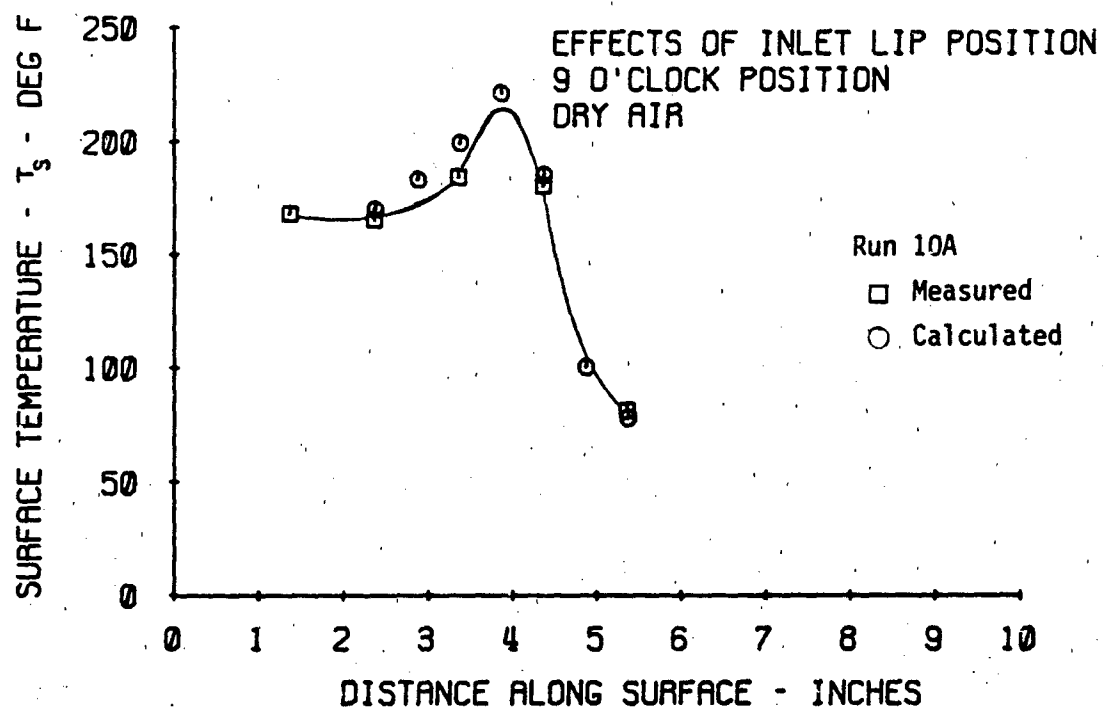
Figure 4-4 Comparison of Calculated and Measured Surface Temperature
