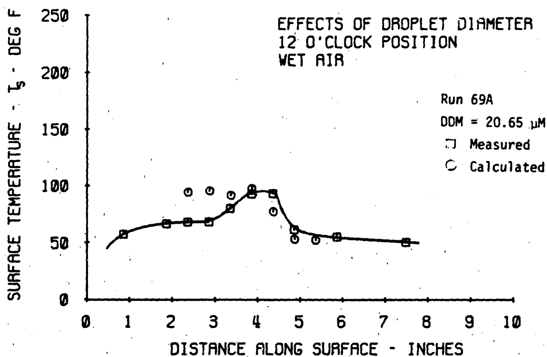
Figure 4-19 Comparison of Calculated and Measured Surface Temperature for Different Water Droplet Diameters. - Single skin.
