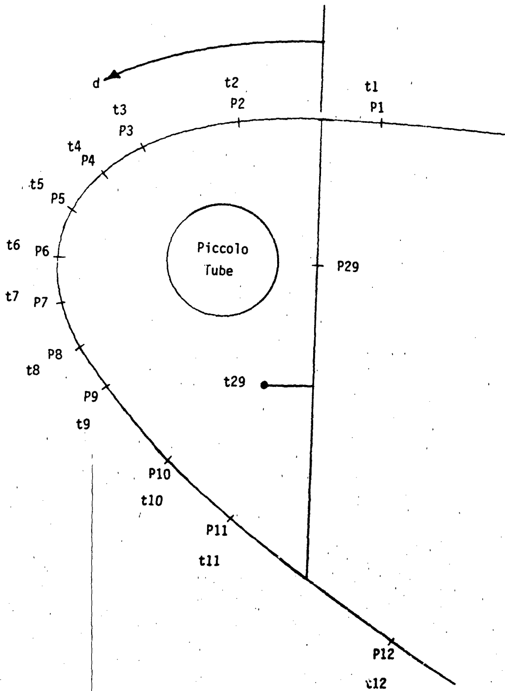
Figure 3-2 Typical Instrumentation Points on Nacelle Inlet Lip - 6 O'clock Position
