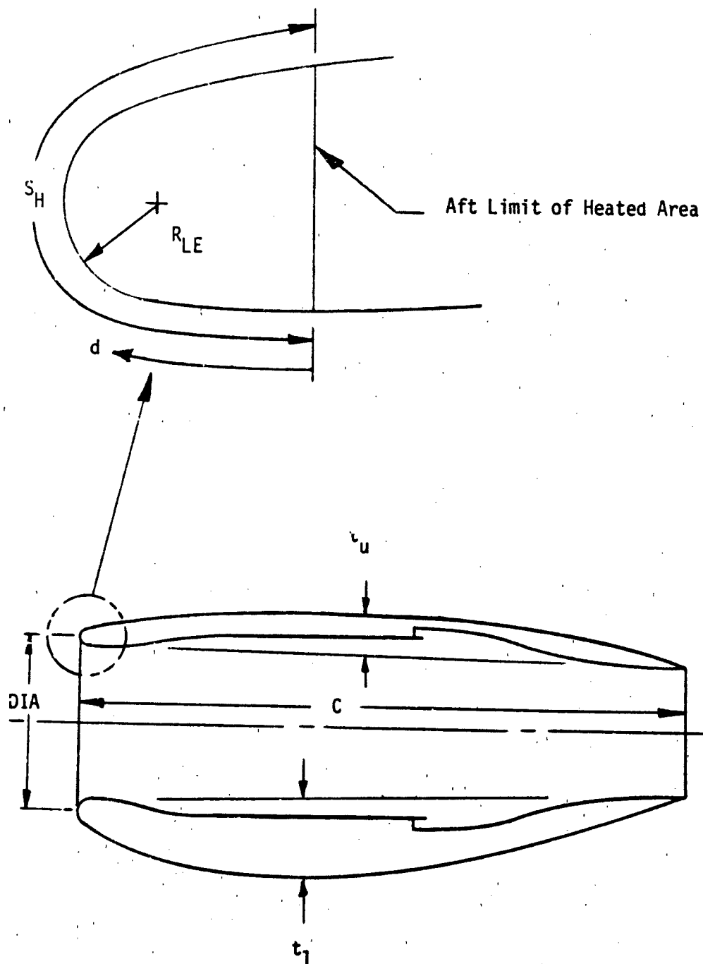
FIGURE 2-1 Nacelle Configuration Definition
