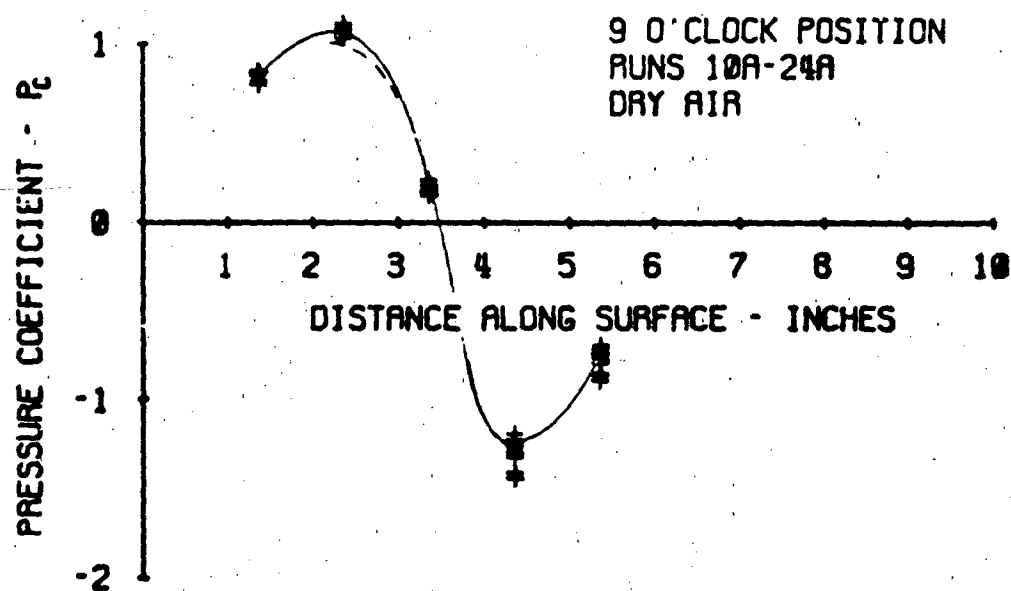
Figure 4-1. Averaged Surface Pressure Coefficients
