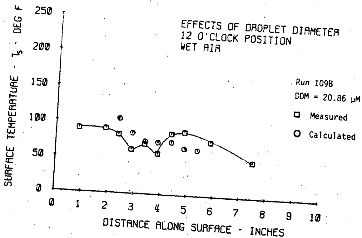
Figure 4-19 - (Cont.) - Double Skin
