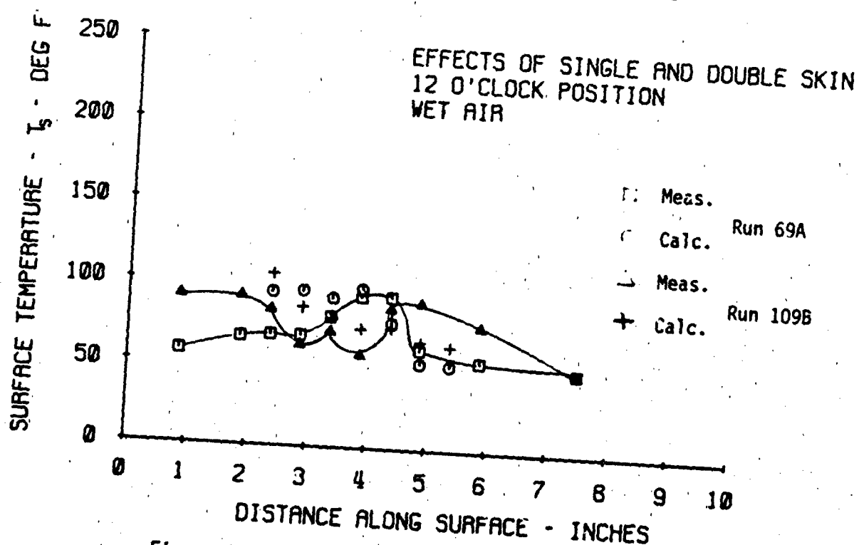
Figure 4-15 Comparison of Calculated and Measured Surface Temperature for Single and Double Skin Distribution Systems.
