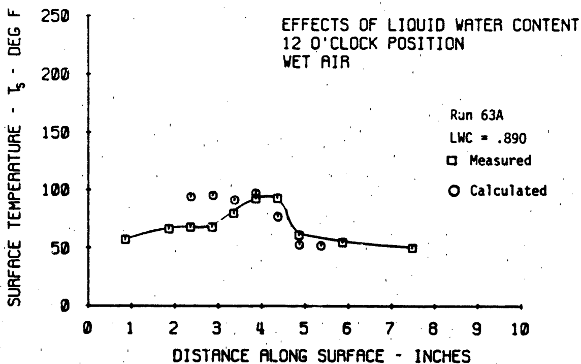
Figure 4-18 Comparison of Calculated and Measured Surface Temperature for Different Liquid Water Content.
