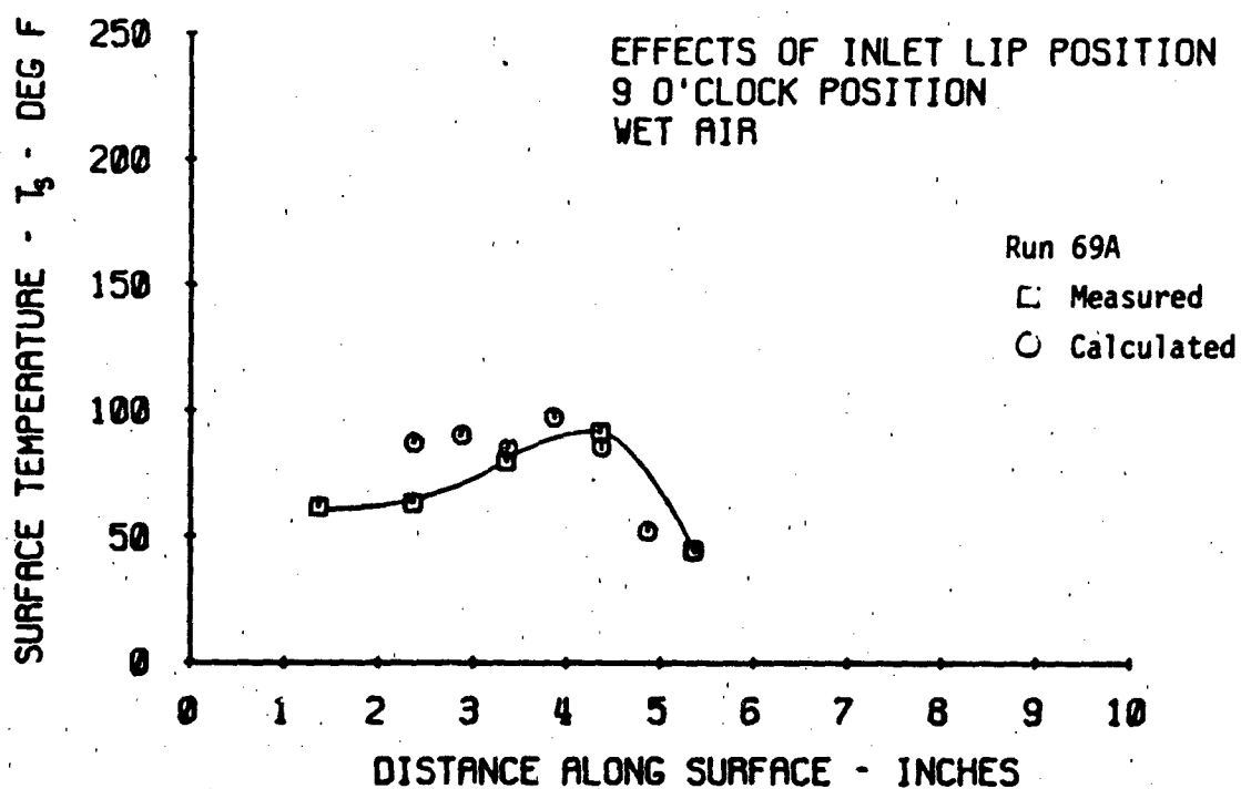
Figure 4-7 Comparison of Calculated and Measured Surface Temperature for Three Nacelle Lip Positions.
