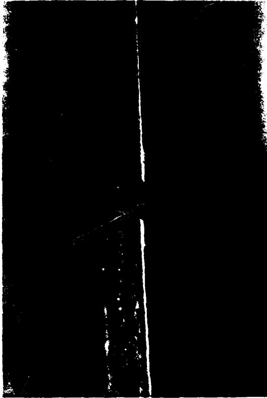
Figure 9. Backer rod of foam.
