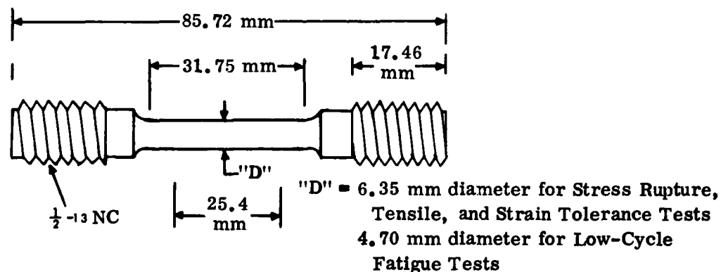
Figure 3. Test Specimen for Strain Tolerance, Low-Cycle Fatigue and Stress-Rupture Tests
