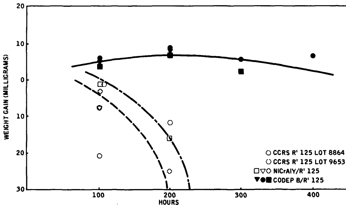
Figure 48. Weight Gain Curve for Coated Rene' 125 Tested in 1149°C (2100°F) Dynamic Oxidation (GE Data)
