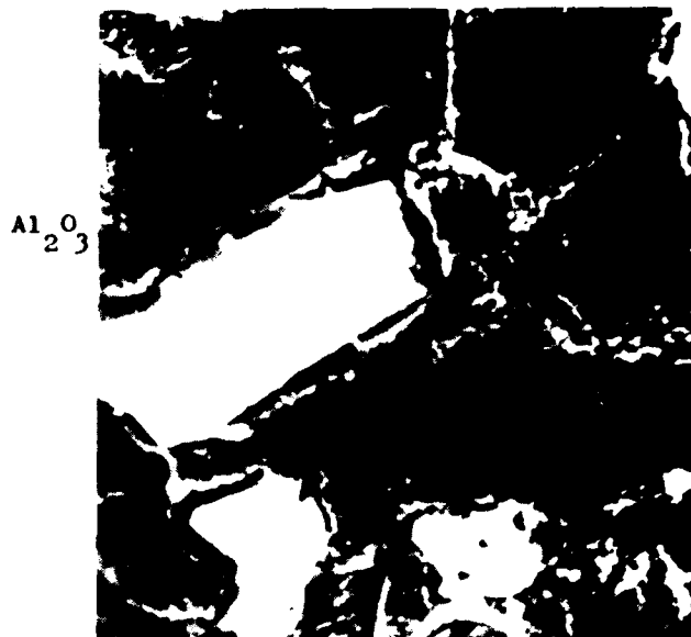
Figure B-15. SEM Shot of Surface of a Dense CCRS CoNiCrAlY Coated Rene' 125 Stress-Rupture Specimen After Test Showing Large Amounts of Entrapped Surface Alumina and Severe Surface Cracking (Arrows)
