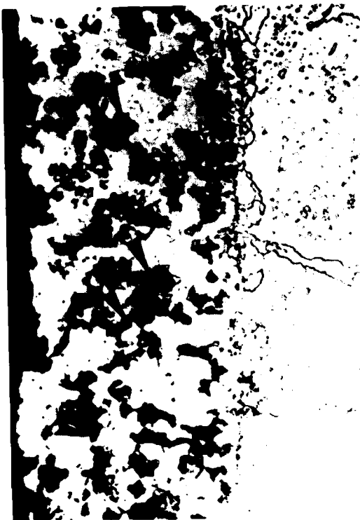
Figure B-17. Typical CCRS CoNiCrAlY/X-40 Stress Rupture Specimen Tested at 1800°F at 11 Ksi Showing (A) Coating Voids and (B) Preferential Oxidation Near Coating Alpha-Chromium Particles and Voids
