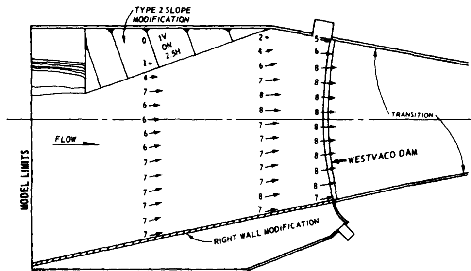
PLAN (7 FT ABOVE CHANNEL INVERT)
