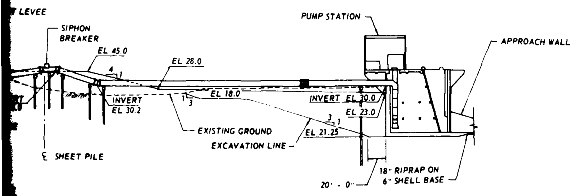
PLAN AND PROFILE PROPOSED DESIGN
