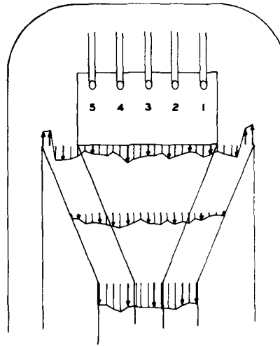
e PUMPS 1-5 OPERATING, TW EL 217 FT
