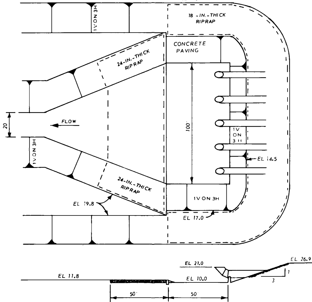
Figure 11. Type 3-modified (recommended) design stilling basin, 45-degree saxophone outlets
