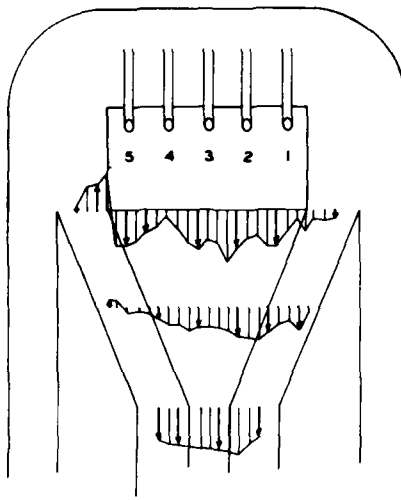
c PUMPS 1-3 OPERATING, TW EL 190 FT
