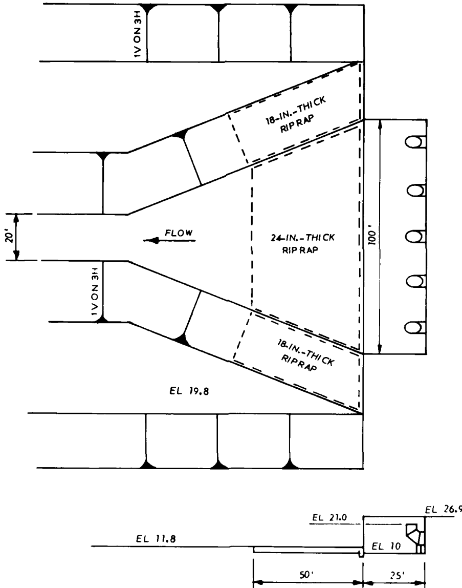
Figure 10. Type 2-modified stilling basin, 90-degree saxophone outlets
