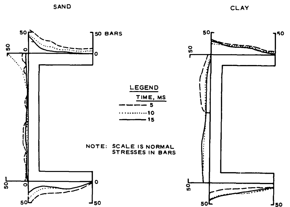
a. INSTANTANEOUS NORMAL STRESSES
