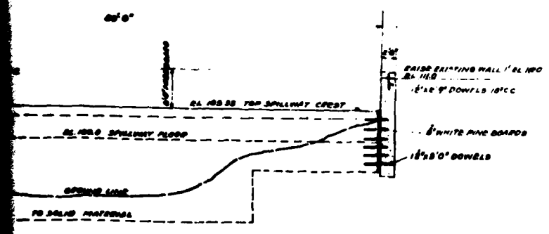
SECTION C-C Scale 1/4" = 1'-0"
