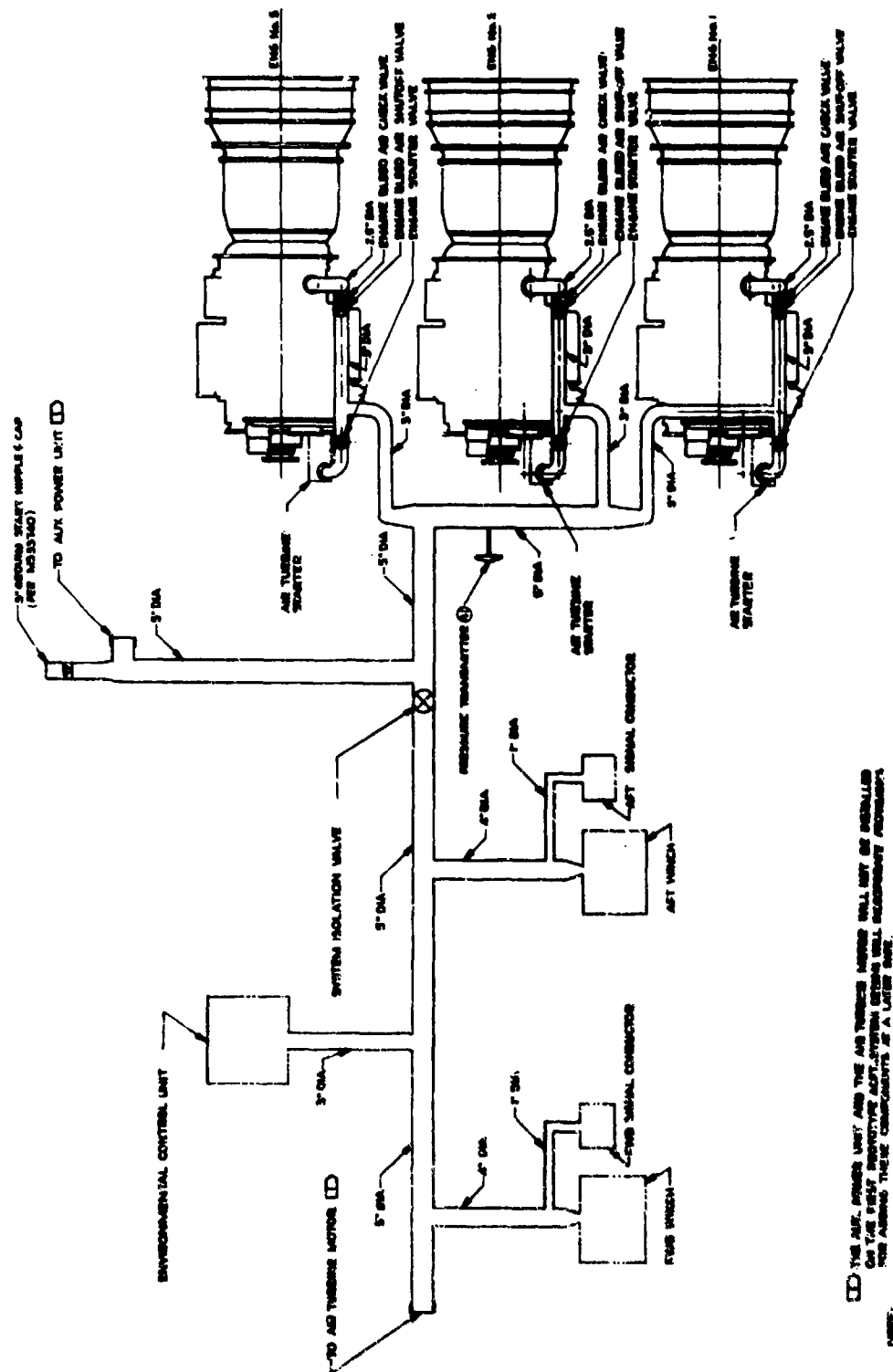
Figure 107. Pneumatic system supply schematic.
