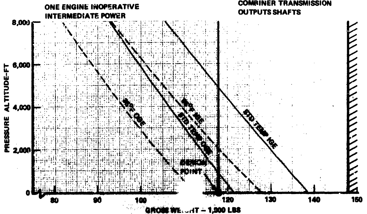
Figure 16. Hover ceiling.
