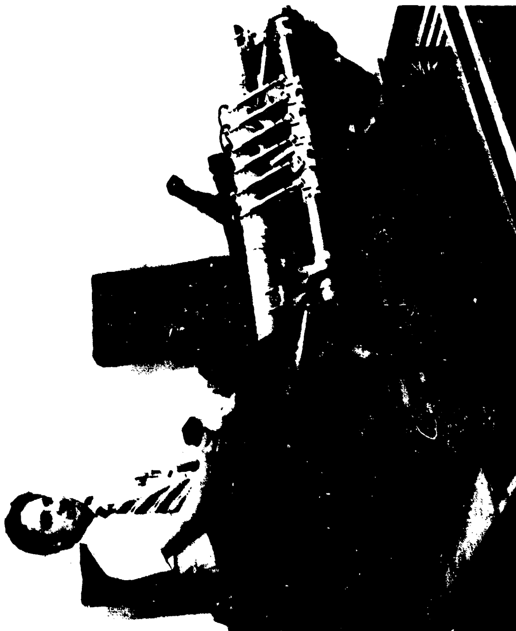
Figure 141. Cockpit control system.
