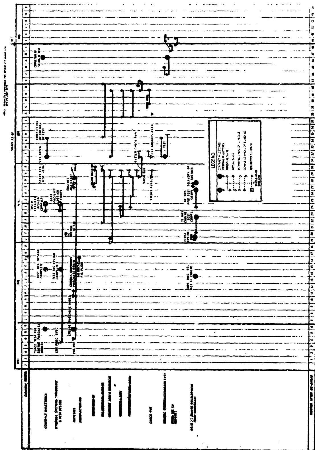
Figure 5A. Integrated rotor/drive system demonstration tests.
