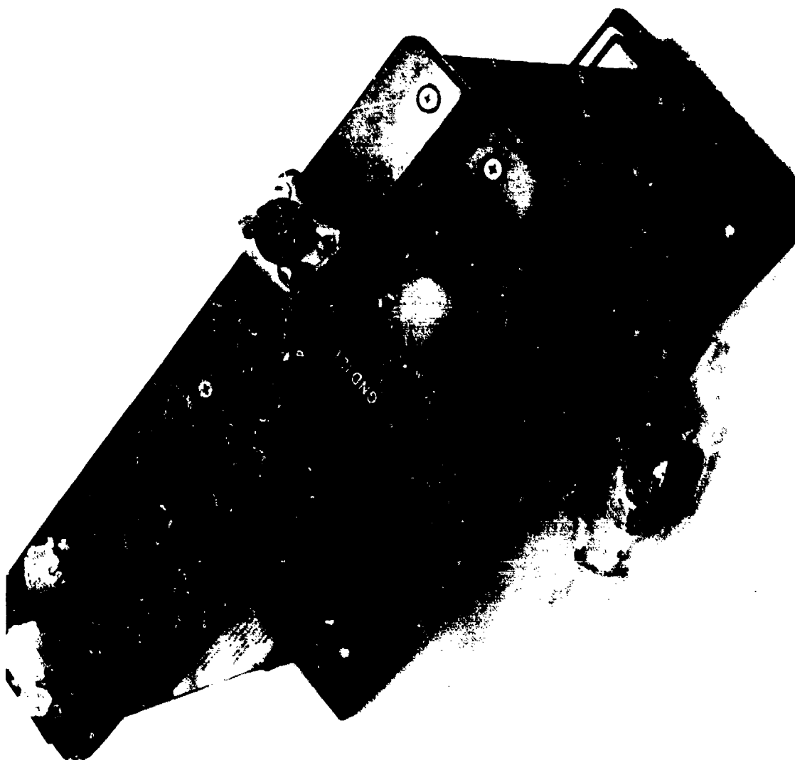
Figure 91. Brassboard control quadrant.
