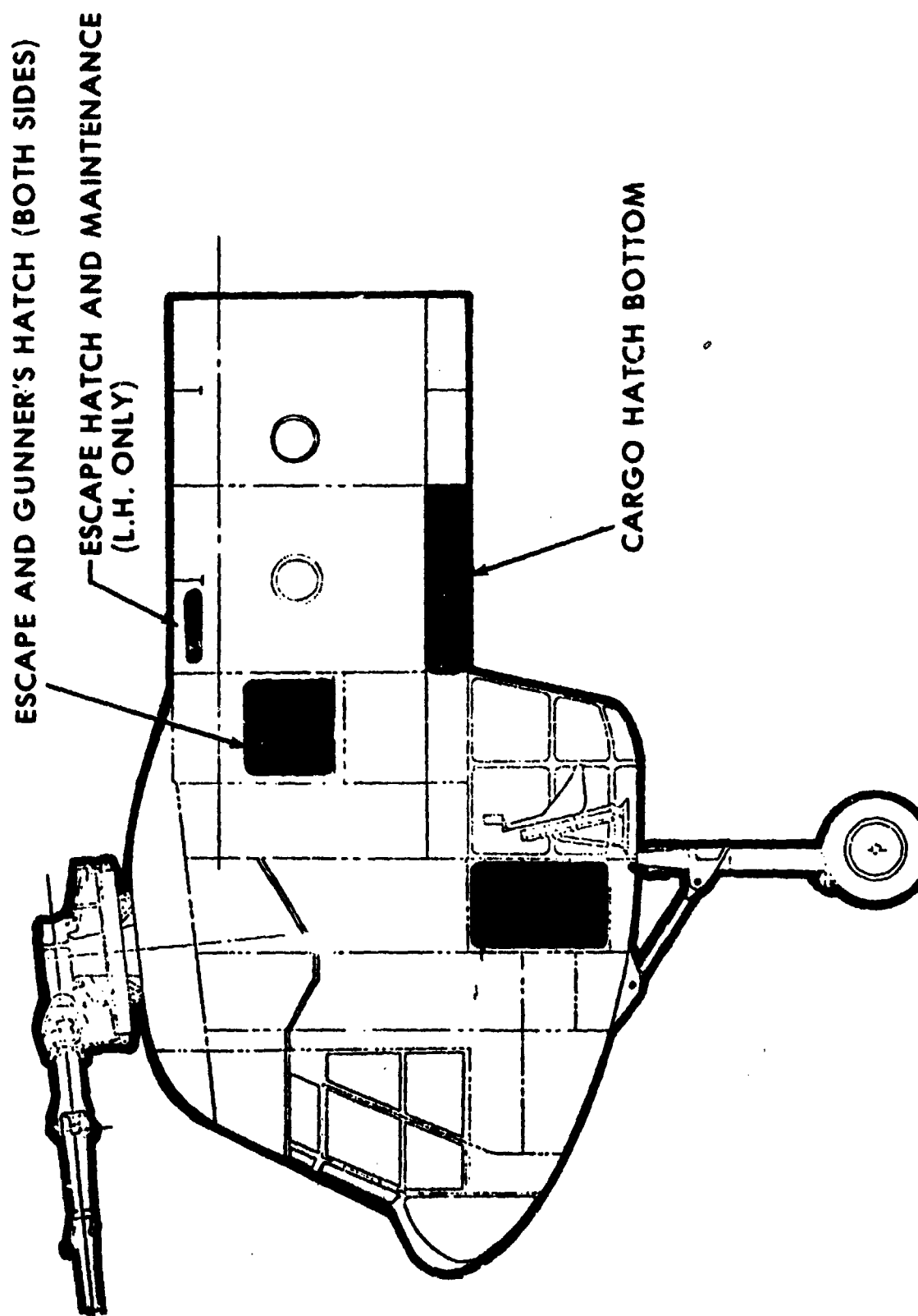
Figure 28. Initial structural arrangement.
