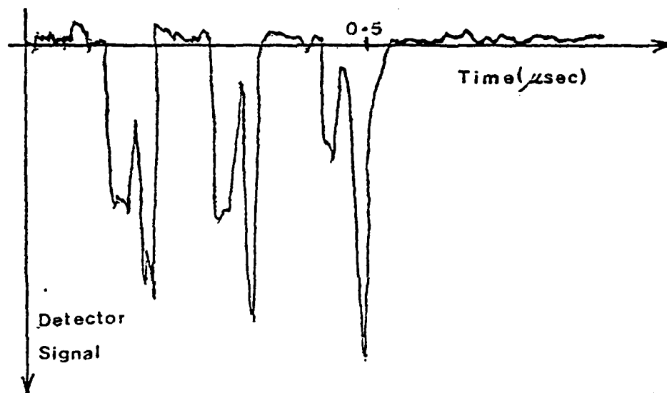
Fig. 3. Crystal detector outputs from two magnetic pickup loops located at different axial positions in the drift tube. The first two peaks represent the pickup signals and the third shows the interference pattern obtained by combining the two signals.
