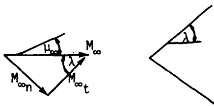
Swept Wing Viewed from Above
