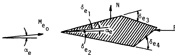
wing cross section normal to leading edge
