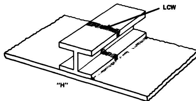
FIGURE 1 CROSS SECTIONAL CONFIGURATIONS OF TYPICAL LONGITUDINAL STIFFENERS
