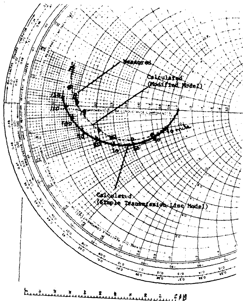
Fig. 7. Measured and Calculated Reflection Coefficients for METCHIPs at 9.35 GHz
