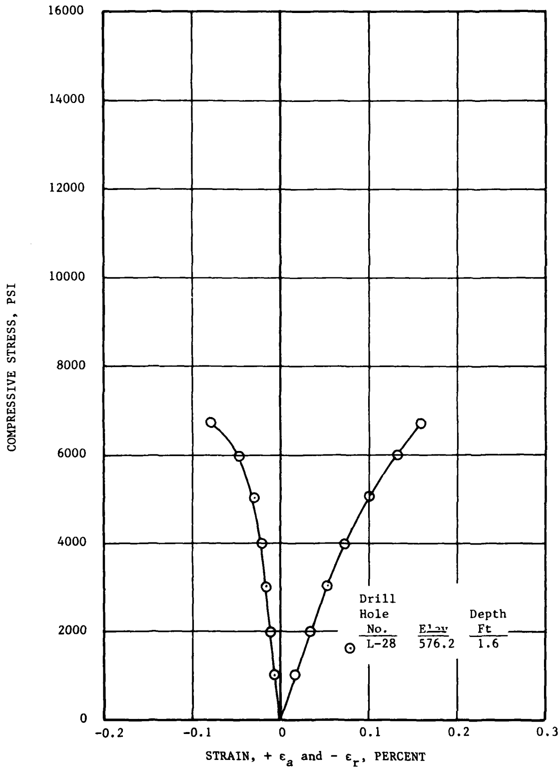
Stress-strain relation for concrete (horizontal hole) upper approach wall, Lockport Lock. PLATE 18
