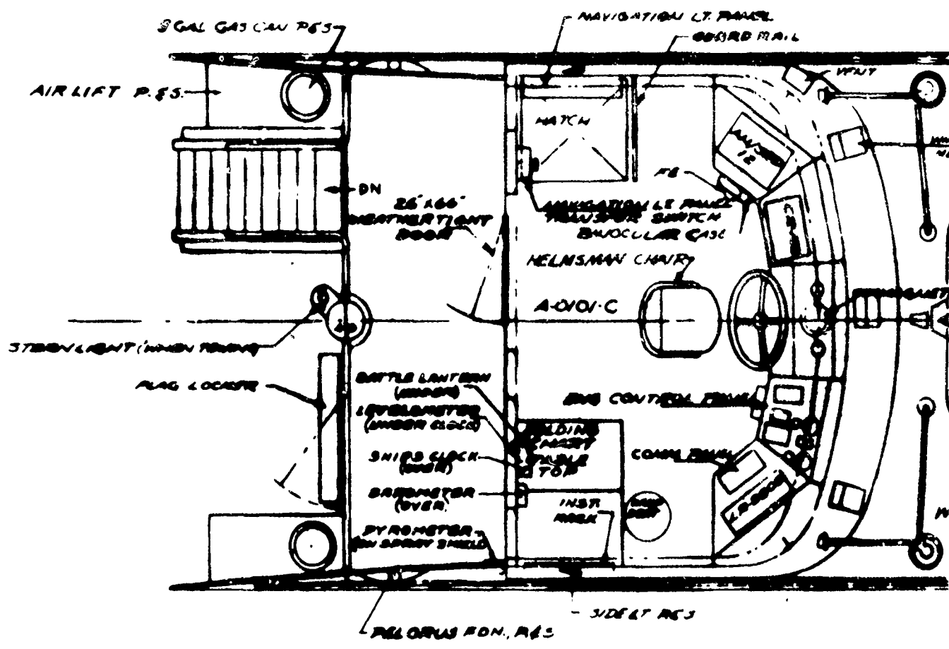
PLAN WHEELHOUSE AND CABIN TOP
