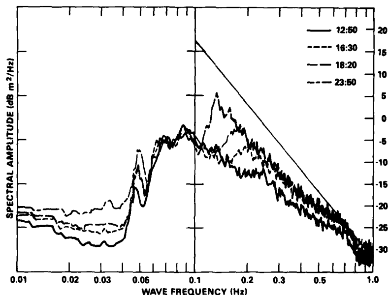
Fig. 14. Four different ocean wave spectra are plotted on a log-log scale for the times indicated, using a 2 mHz frequency resolution, and with each plot the result of 1-h incoherent averaging. Equation (7), with \alpha = 0.008 , is plotted as a straight line. The broad band of wave energy from 0.06 Hz and higher is the result of energy which had propagated from the west from a storm at sea some 200 miles away. Wave energy at frequencies above 0.1 Hz which shows a changing character from one time period to the next is the result of local winds blowing from 310 to 320 deg bearing over the time periods indicated.
