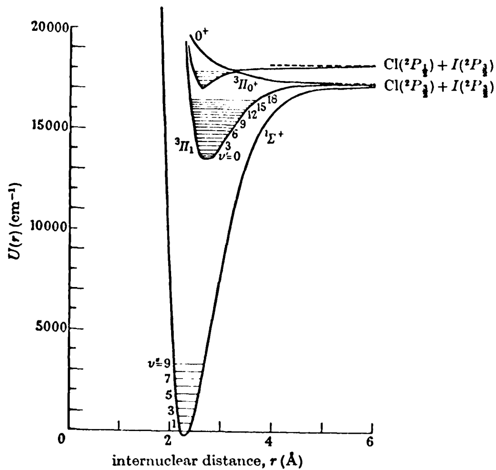
Figure 4. Morse Potential Energy Functions for ICl
