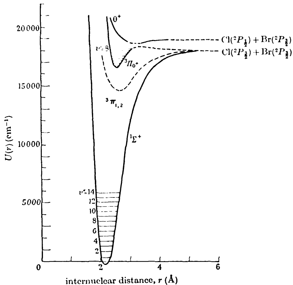
Figure 5. Morse Potential Energy Functions for \text{BrCl} (Broken Lines Indicate the Estimated Positions of Unobserved States.)
