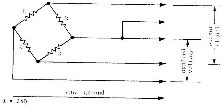
(b) Electrical details.
