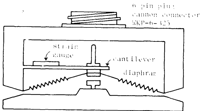
(a) Mechanical details.
