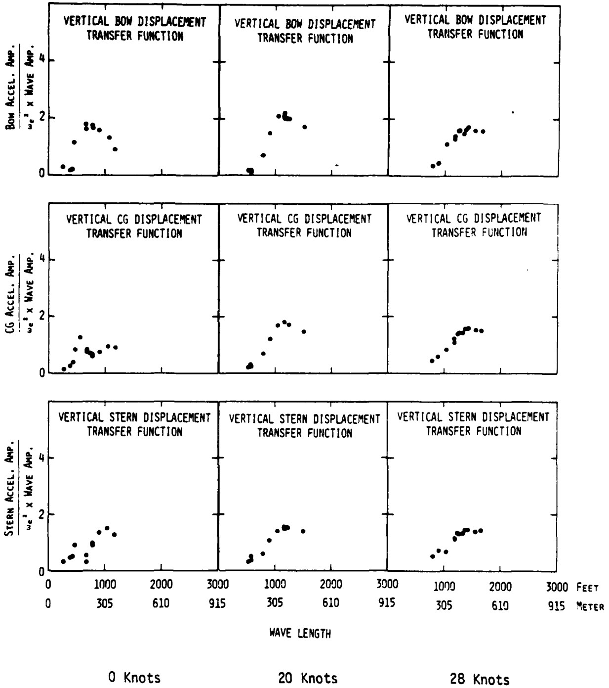
Figure 8 - Vertical Displacement Transfer Functions in Regular Head Seas for SWATH 6C
