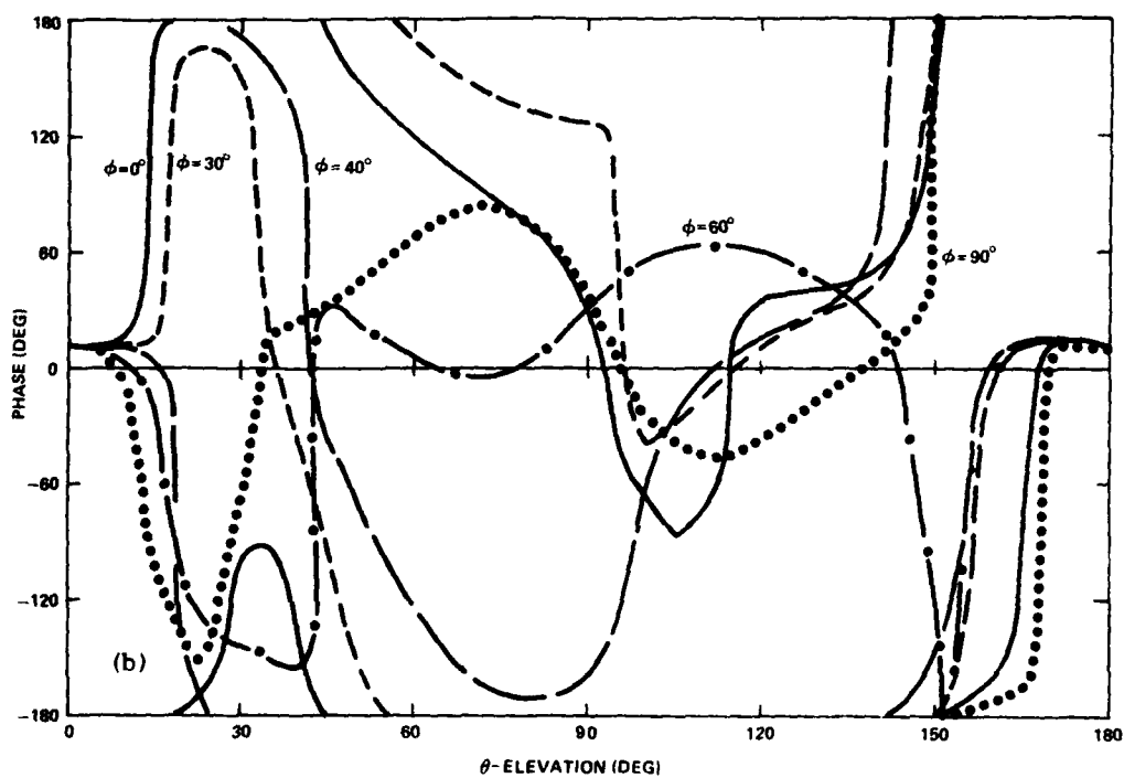
Figure 6. Twenty-eight-MHz Elevation Plane Backscatter Field Phase Values for a = 0.00096 m: (a) E_\phi polarization; (b) E_\theta polarization
