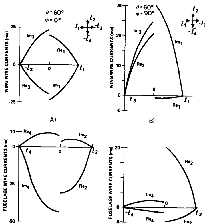
Figure 26. Complex Currents Induced on the Wires in Method-of-Moment Solution for a 7-MHz, E_\theta Polarized Signal, and Elevation Angle \theta = 60^\circ . Arrows indicate direction convention for positive current at; (a) azimuthal angle \phi = 0^\circ and (b) azimuthal angle \phi = 90^\circ
