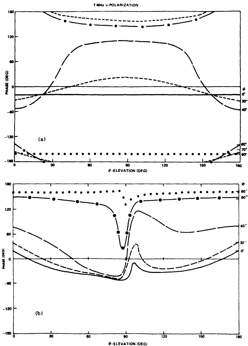
Figure 4. Seven-MHz Elevation Plane Backscatter Field Phase Values for a = 0.0019 m: (a) E_\phi polarization and (b) E_\theta polarization
