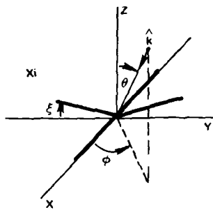
Figure 23. Scattering Model Configuration for the Dipole Theory Showing Scattering Angles (\theta, \phi) and Cyclic Wing-Dipole Displacement Angle (\xi)
