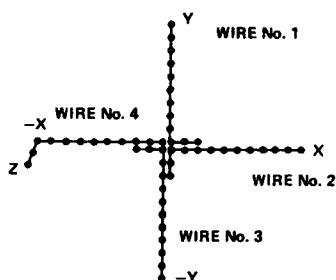
Figure 1. Crossed Wire Configuration Showing 7-MHz Point Spacing
