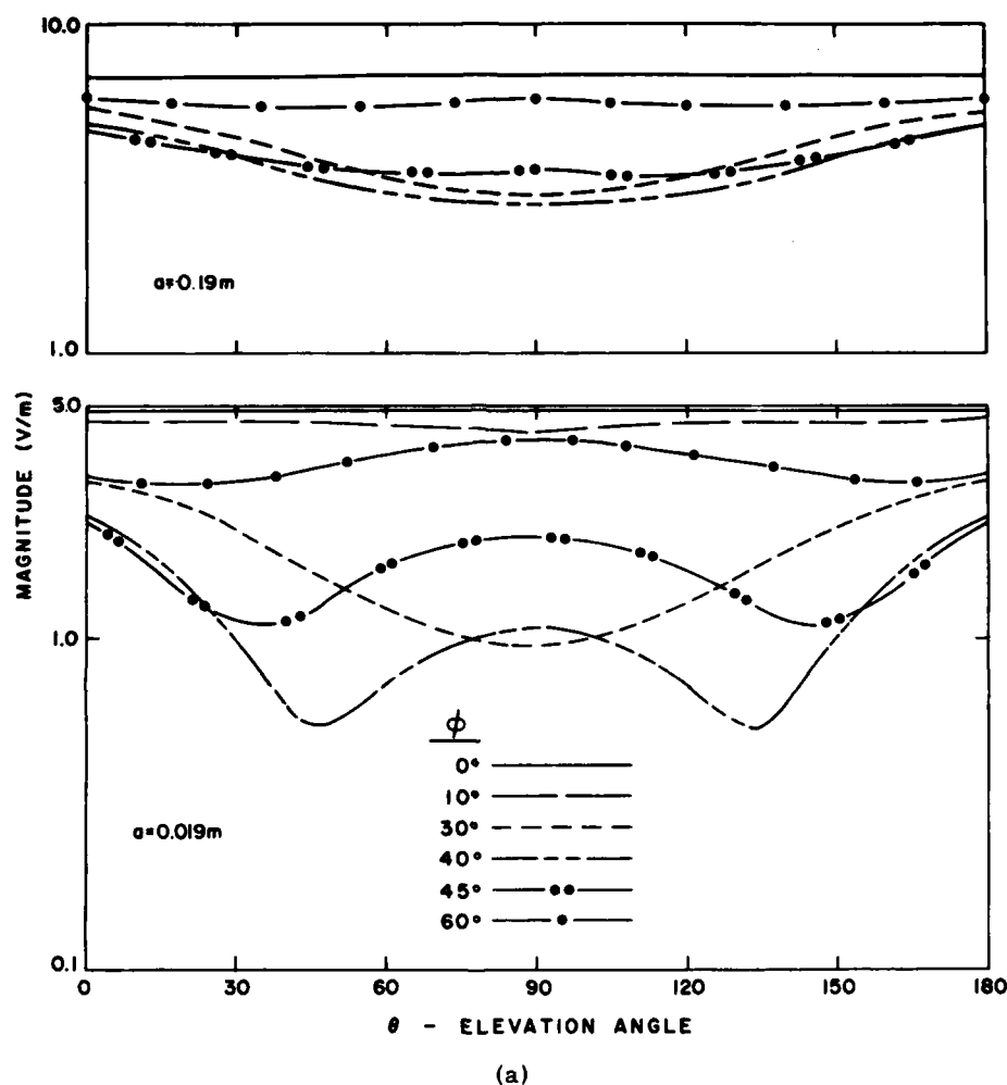
Figure 3. Seven-MHz Elevation Plane Backscatter Field Magnitudes for Successive Values of Wire Radius: (a) E_\phi polarization, a = 0.19 m, and a = 0.019 m; (b) E_\phi polarization, a = 0.0019 m; (c) E_\theta polarization, a = 0.0019 m
