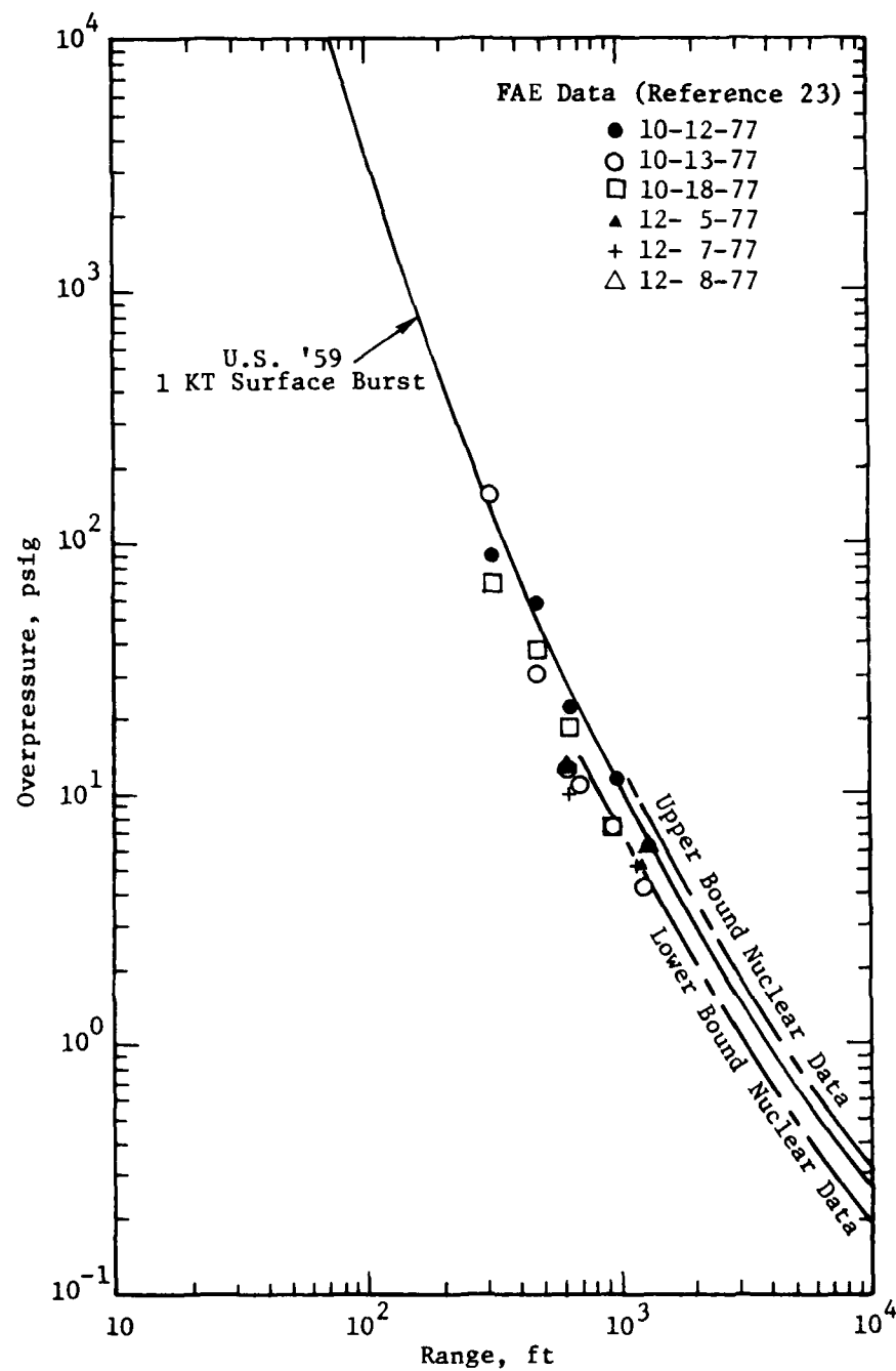
Figure 4.2. FAE peak overpressure data ( S^3 ) scaled to 1 KT surface burst and compared with the U.S. '59 curve.
