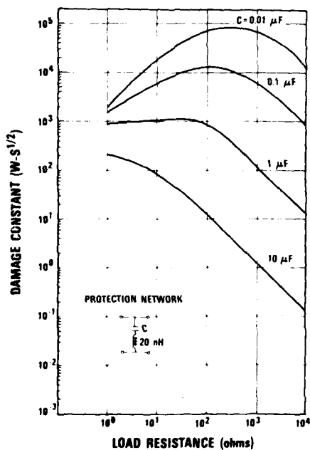
Figure 8. Damage response of circuit load for single-stage filter protection network for following open-wire parameters: 5 km at 5 m, far end shorted, broadside illumination.
