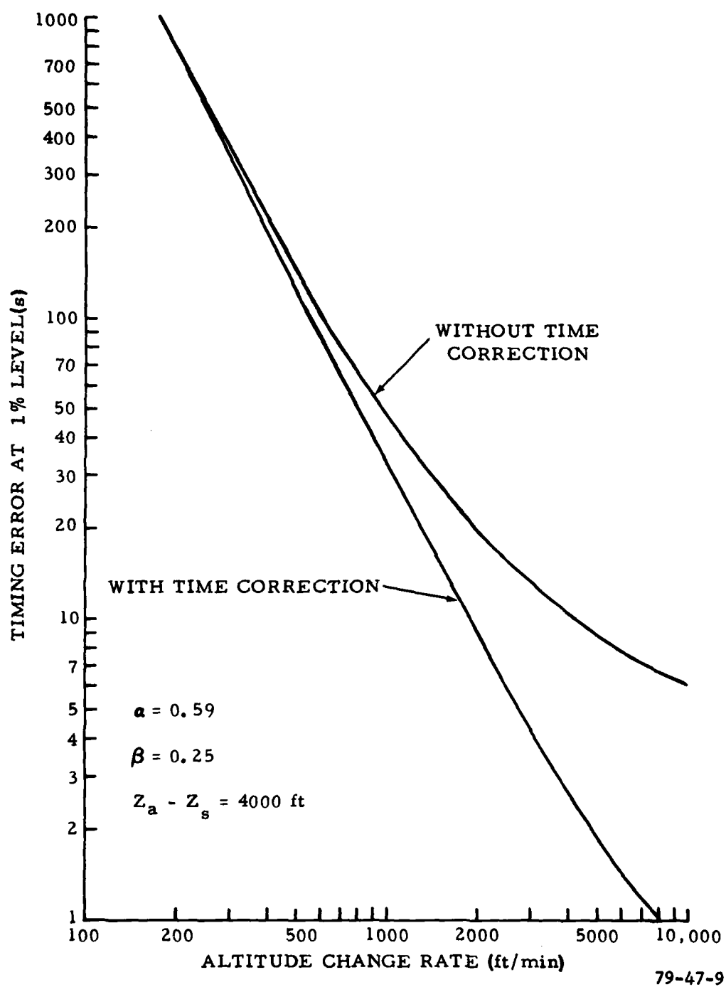
FIGURE 9. TIMING ERRORS AT THE 1-PERCENT LEVEL
