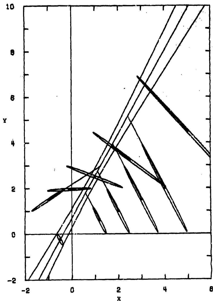
Figure 2b. Falsified Adjustment in x,y -space.
