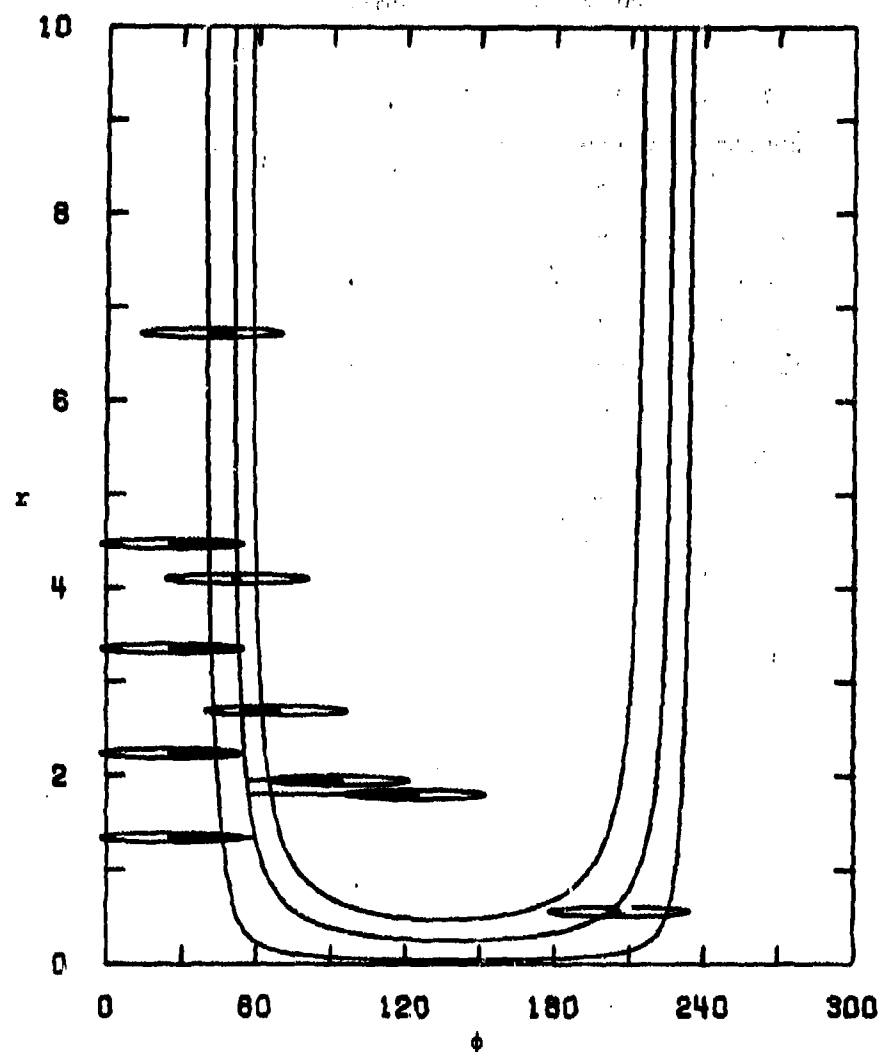
Figure 1a. Adjustment in \phi, r -space.
