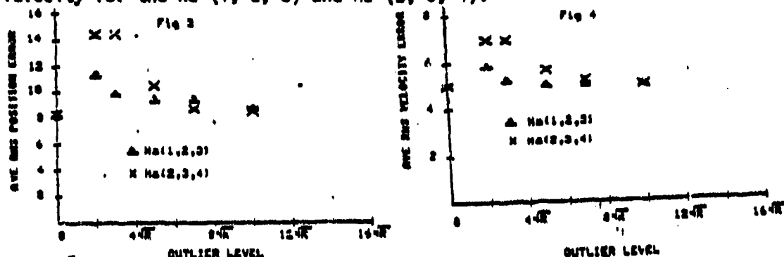
Figures 3 and 4 were made using the same outlier proportions and measurement noise standard deviations as figures 1 and 2.
