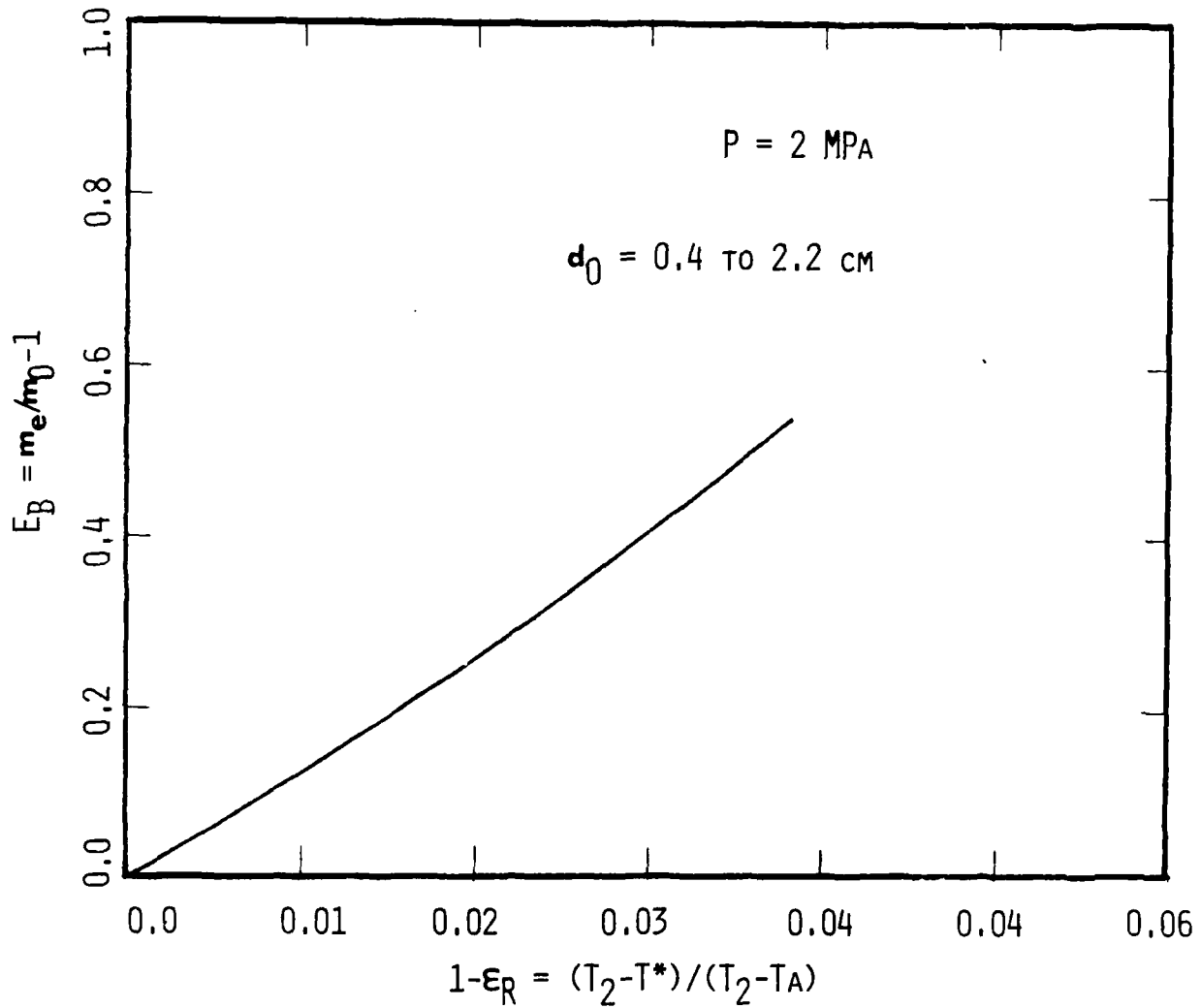
Fig. VI.13 Erosive burning versus reduced cutoff enthalpy at various port diameters ( P = \text{const} ). The erosion effect is self similar with respect to the port diameter, and all the lines coincide.
