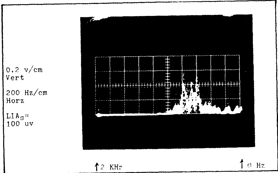
Figure 7.11 Spectral Content of the Closed Loop Error Signal (0 Hz - 2 KHz), Using the G_{c3a} Portion of Compensator G_{c3}
