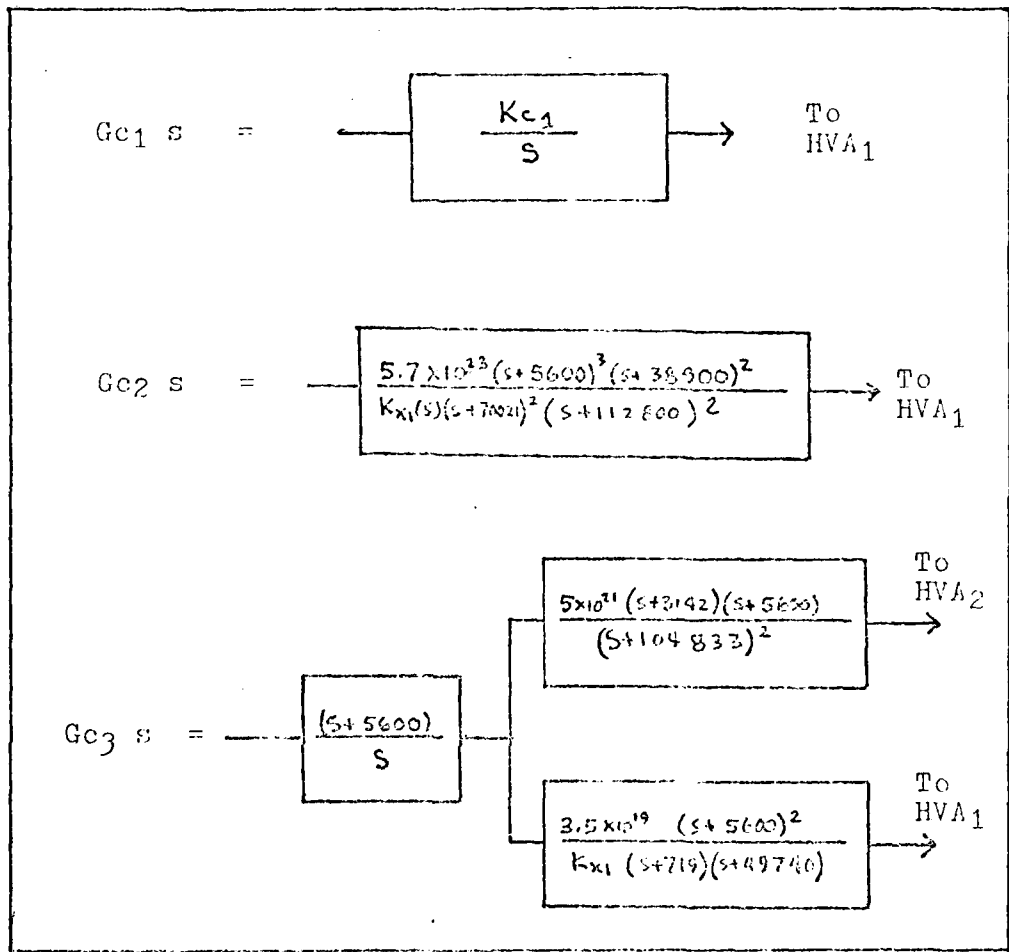
Figure 6.12 Final Compensator Designs
