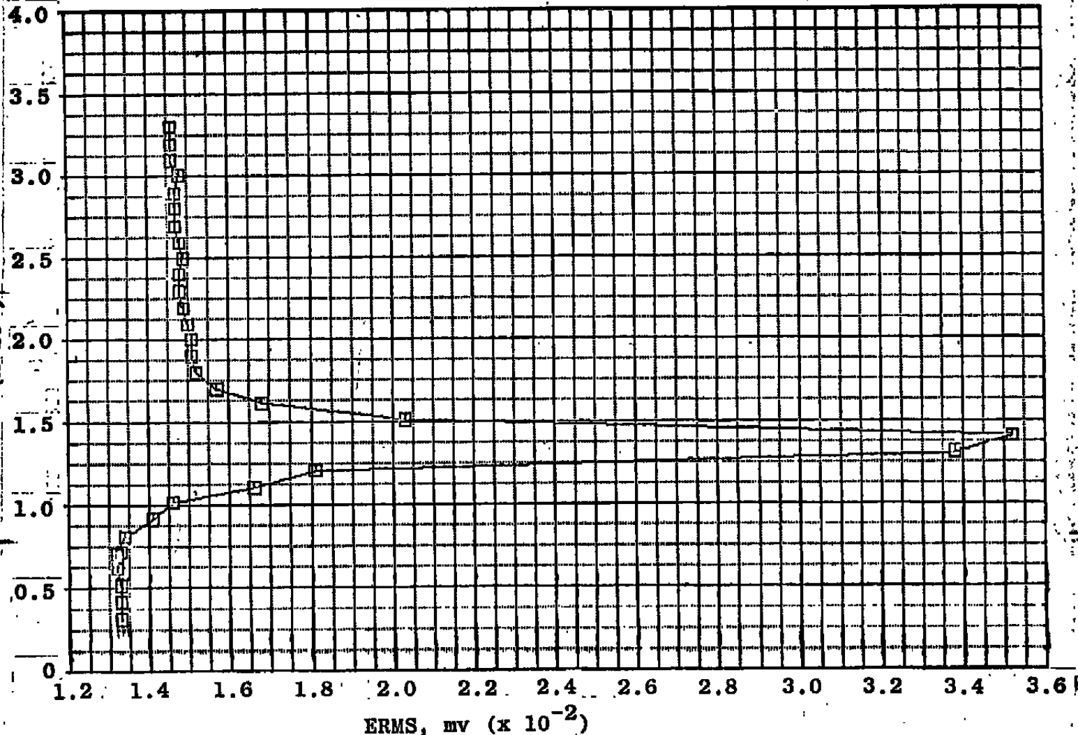
FIG. 10 ILLUSTRATION OF QUALITATIVE HOT-WIRE ANEMOMETER PROFILE RESULTS
