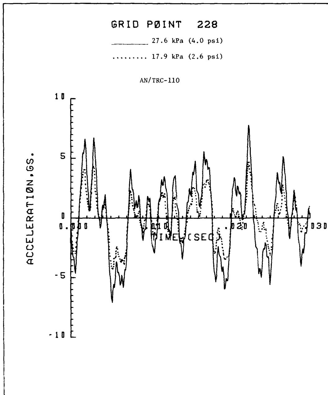
FIGURE 3.30 ACCELERATION TIME HISTORY IN BLAST DIRECTION, FRONT END RACK (NASTRAN)
