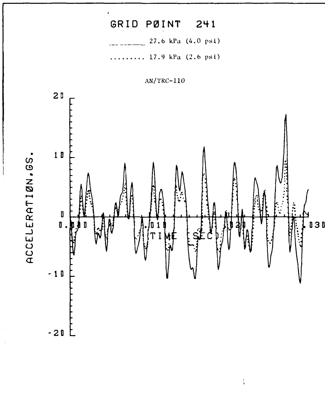
FIGURE 3.32. ACCELERATION TIME HISTORY IN BLAST DIRECTION, FRONT END RACK (NASTRAN)
