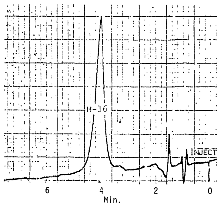
Figure C-4A. HPLC Chromatogram of Reference Compound
