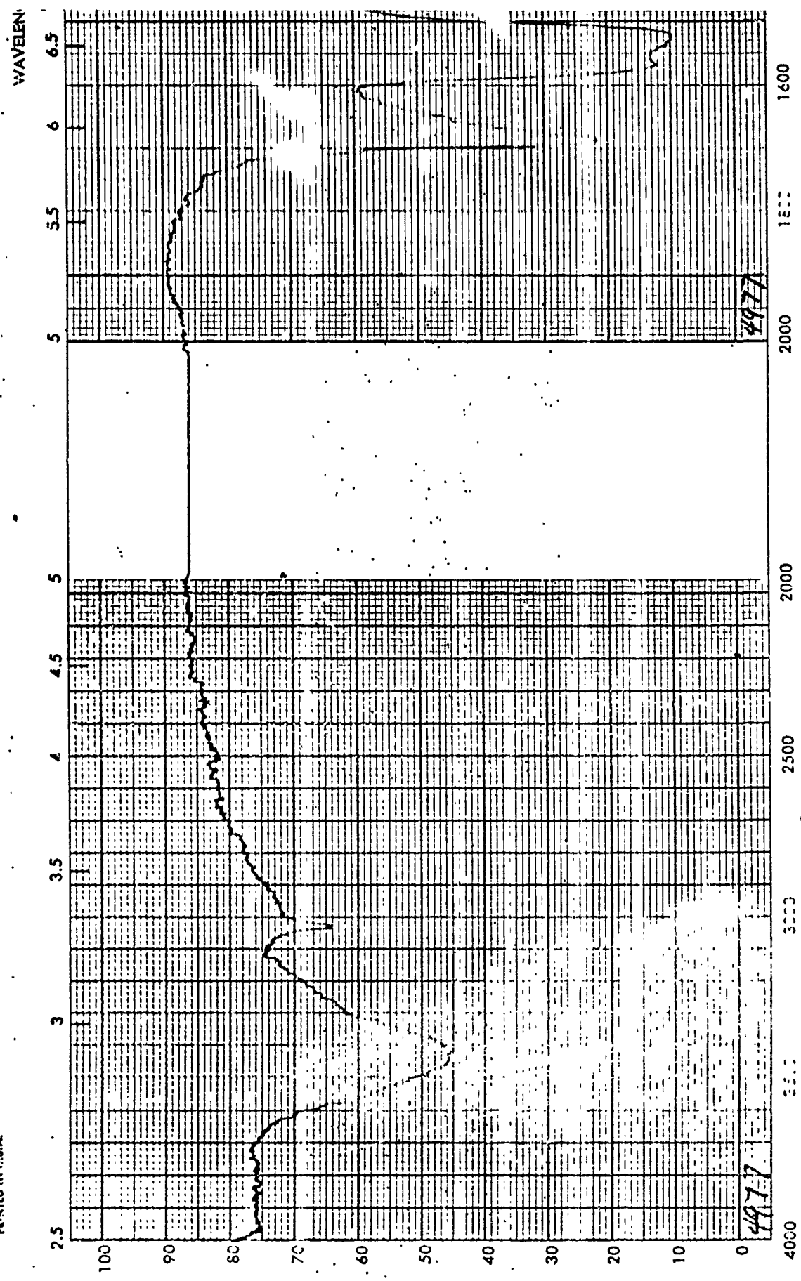
Figure C-14D (Continued). IR Spectrum of RDX Dewater Fraction No. 8
