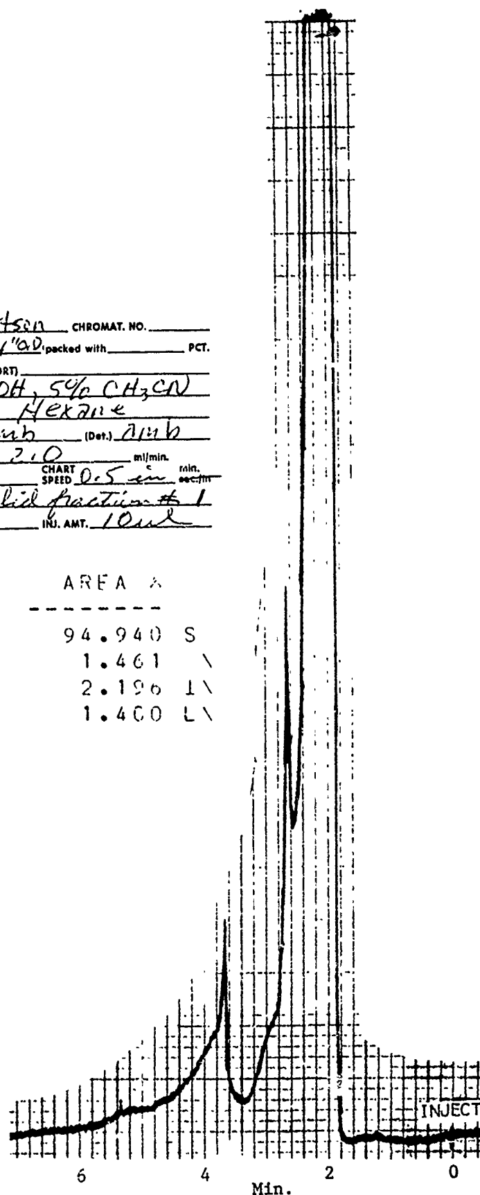
Figure C-9B. HPLC Chromatogram of RDX Dewater Fraction No. 1
