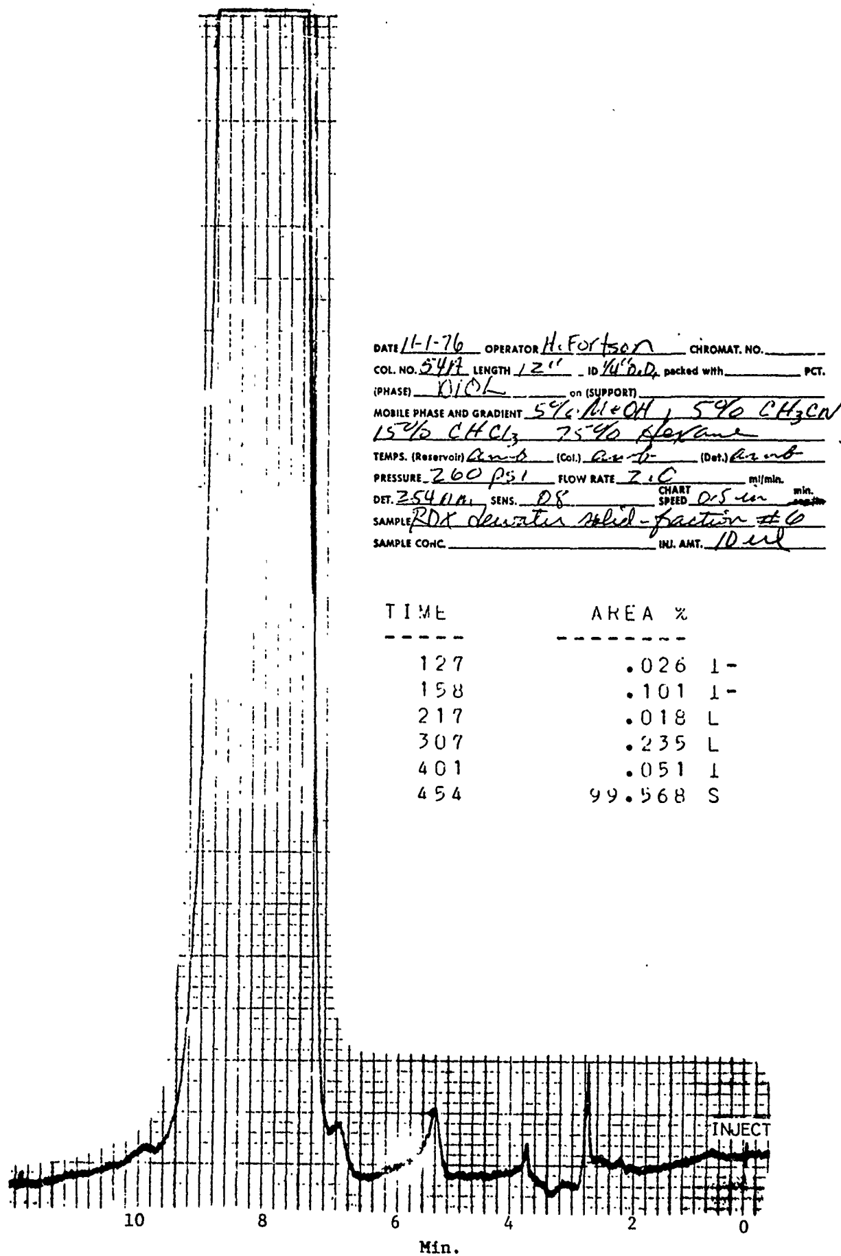
Figure C-14B. HPLC Chromatogram of RDX Dewater Fraction No. 6
