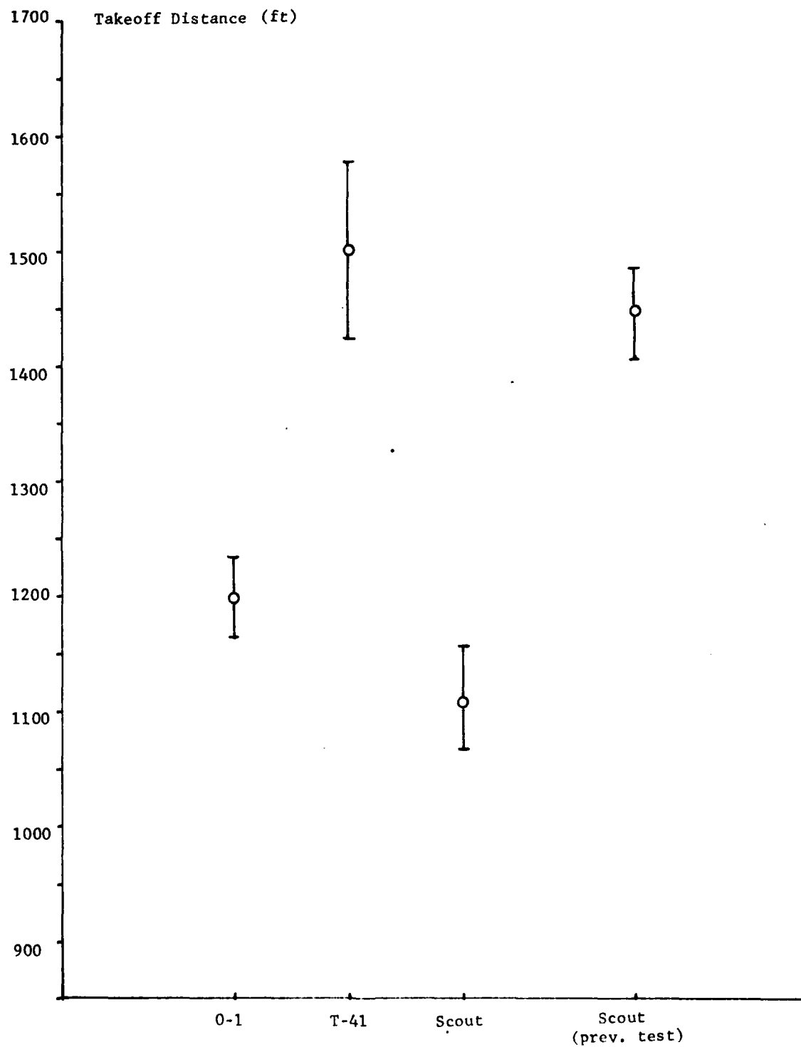
Figure B3. Takeoff Distance Data
