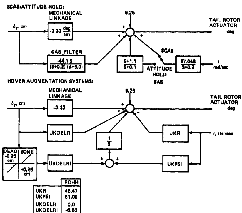
Figure 3. Advanced helicopter control systems - yaw, V < 50 knots.
