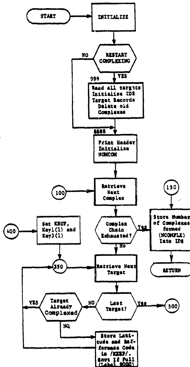
Figure 18. Subroutine COMPLEX (Part 1 of 8)
