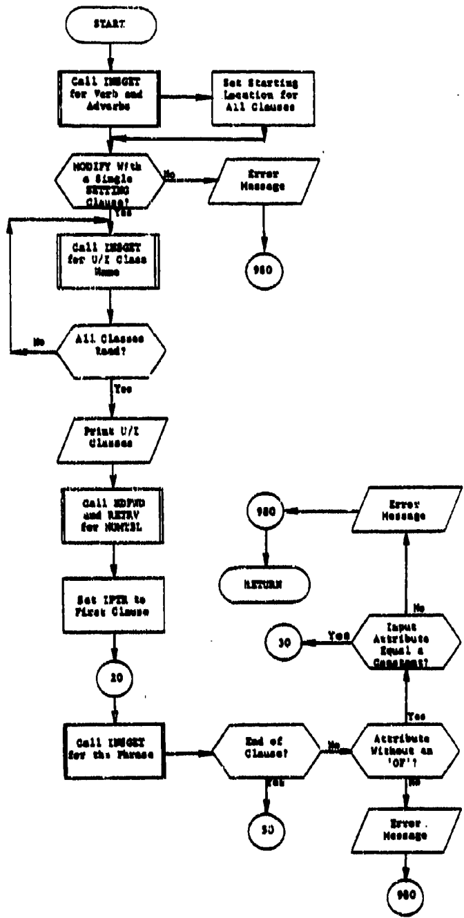
Figure 15. DBMOD Module (Part 1 of 10)
