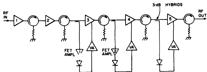
Figure 6. Block diagram showing the modified design.
